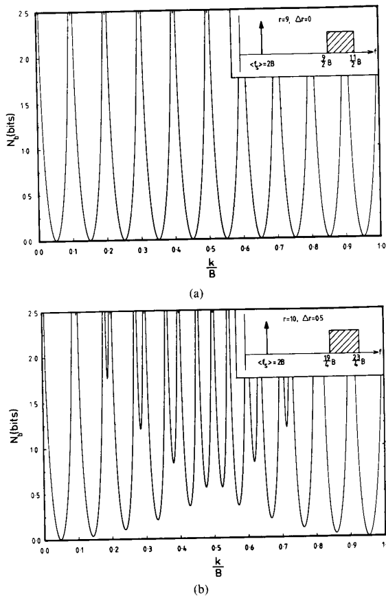
Fig. 8. An estimate of the equivalent number of bits of resolution irrecoverably lost in interpolating a bandpass signal using uncertain baseband rate samples, as a function of k . The graphs represent a cost of a poor choice of k in the second-order bandpass sampling process. The average sample rate is \langle f_s \rangle = 2B . (a) r = 9 , \Delta r = 0 (half-integer band positioning). The minima correspond to cases of quadrature sampling. (b) r = 10 , \Delta r = 0.5 (neither integer nor half-integer band positioning). The minima do not, in general, correspond to quadrature sampling.
