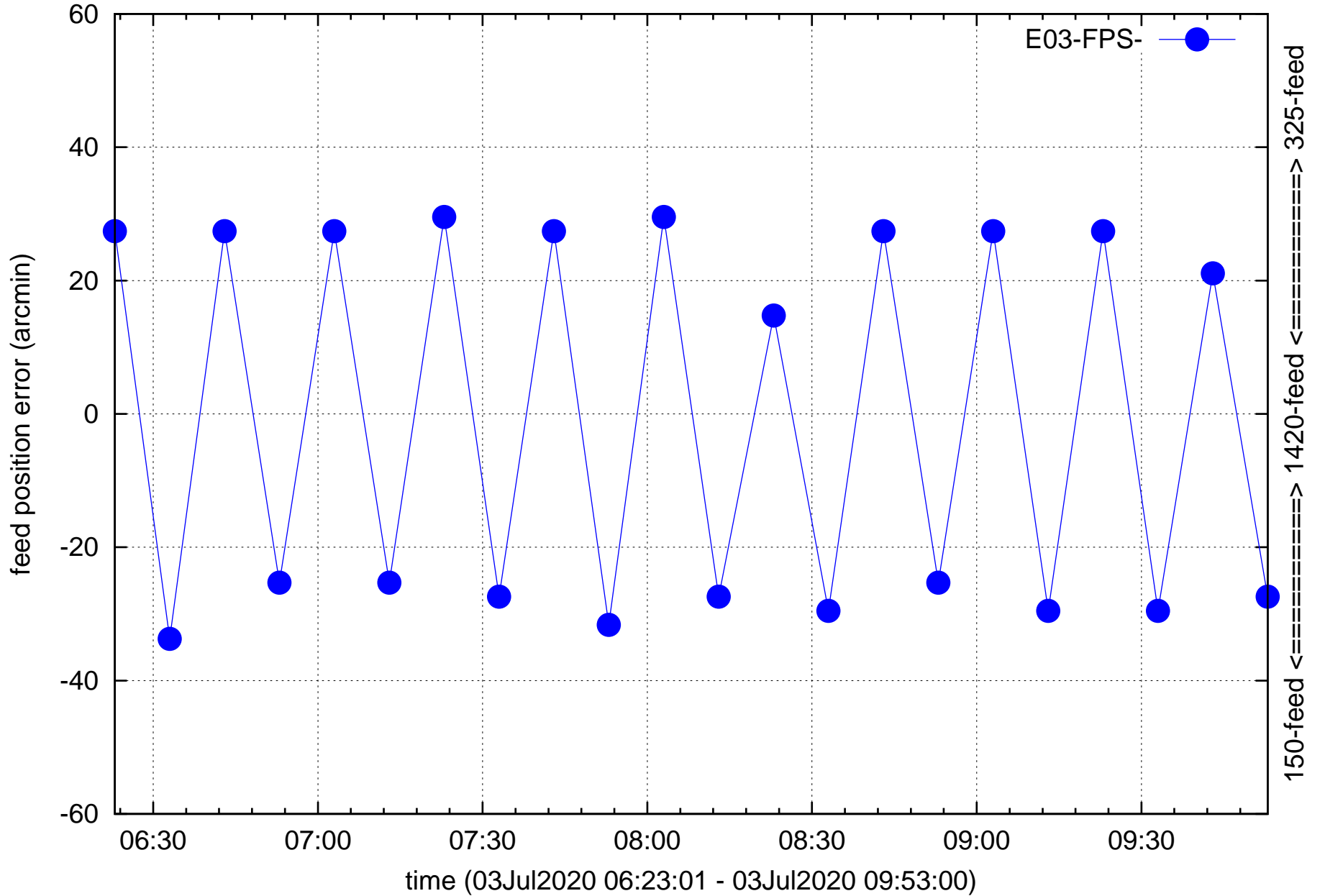
E03 feed refocusing 150=>1420, 325=>1420, ...
