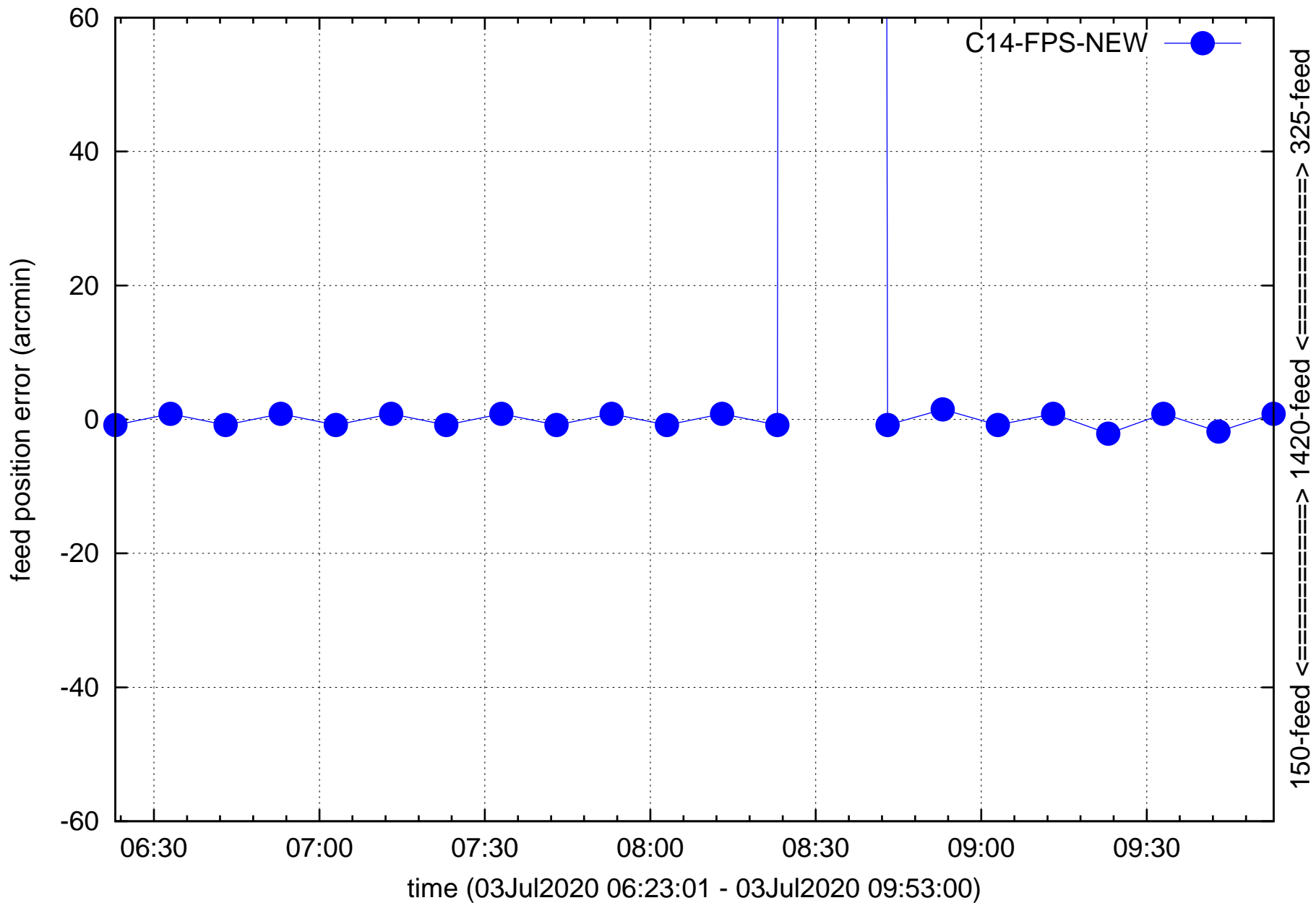
C14 feed refocusing 150=>1420, 325=>1420, ...
