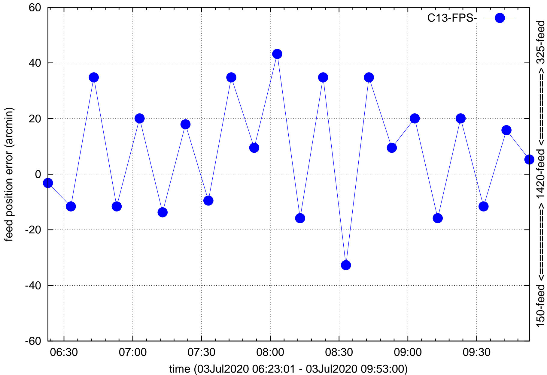
C13 feed refocusing 150=>1420, 325=>1420, ...
