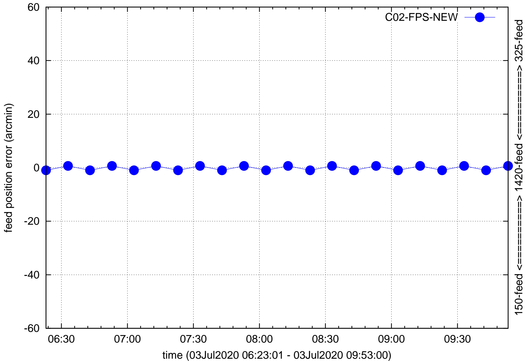
C02 feed refocusing 150=>1420, 325=>1420, ...
