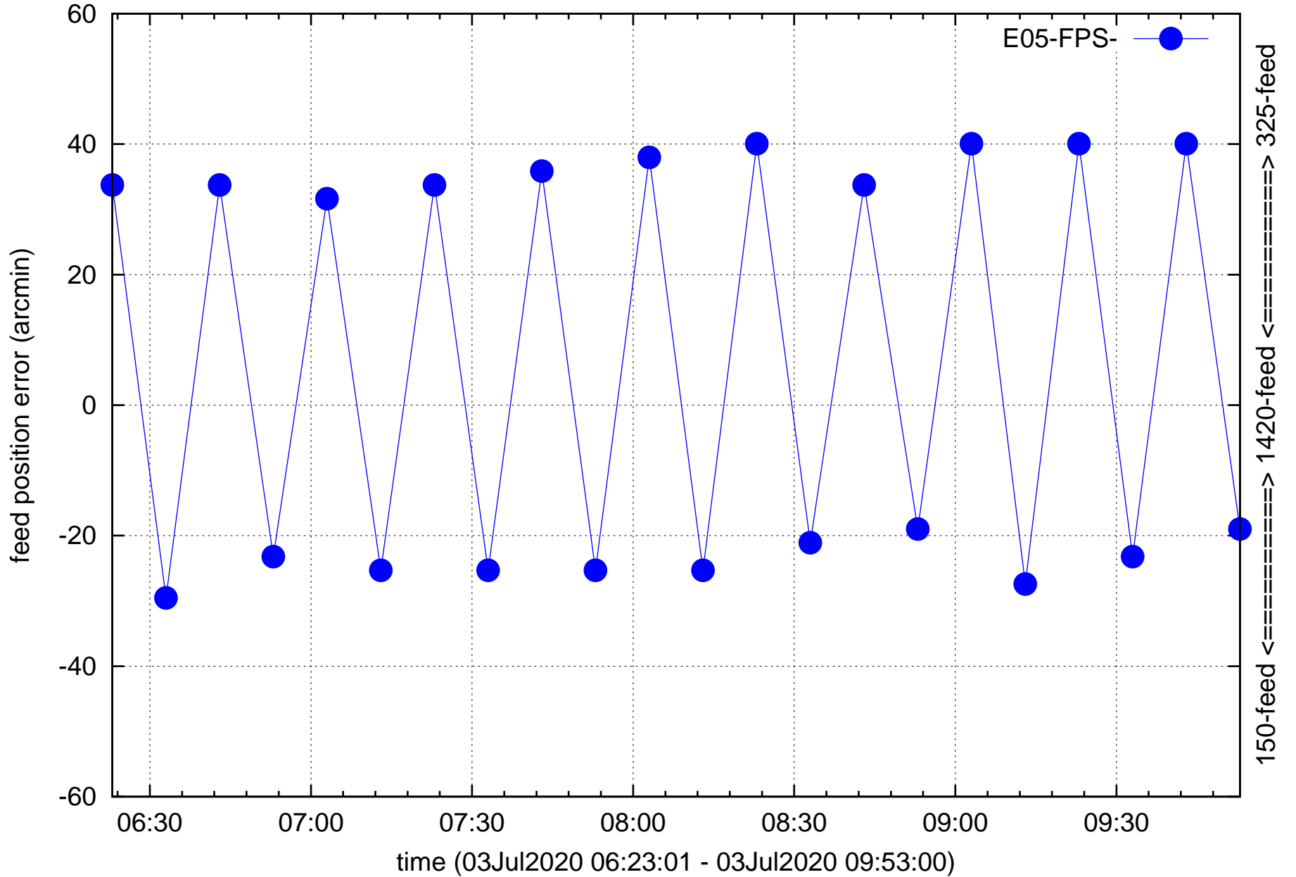
E05 feed refocusing 150=>1420, 325=>1420, ...
