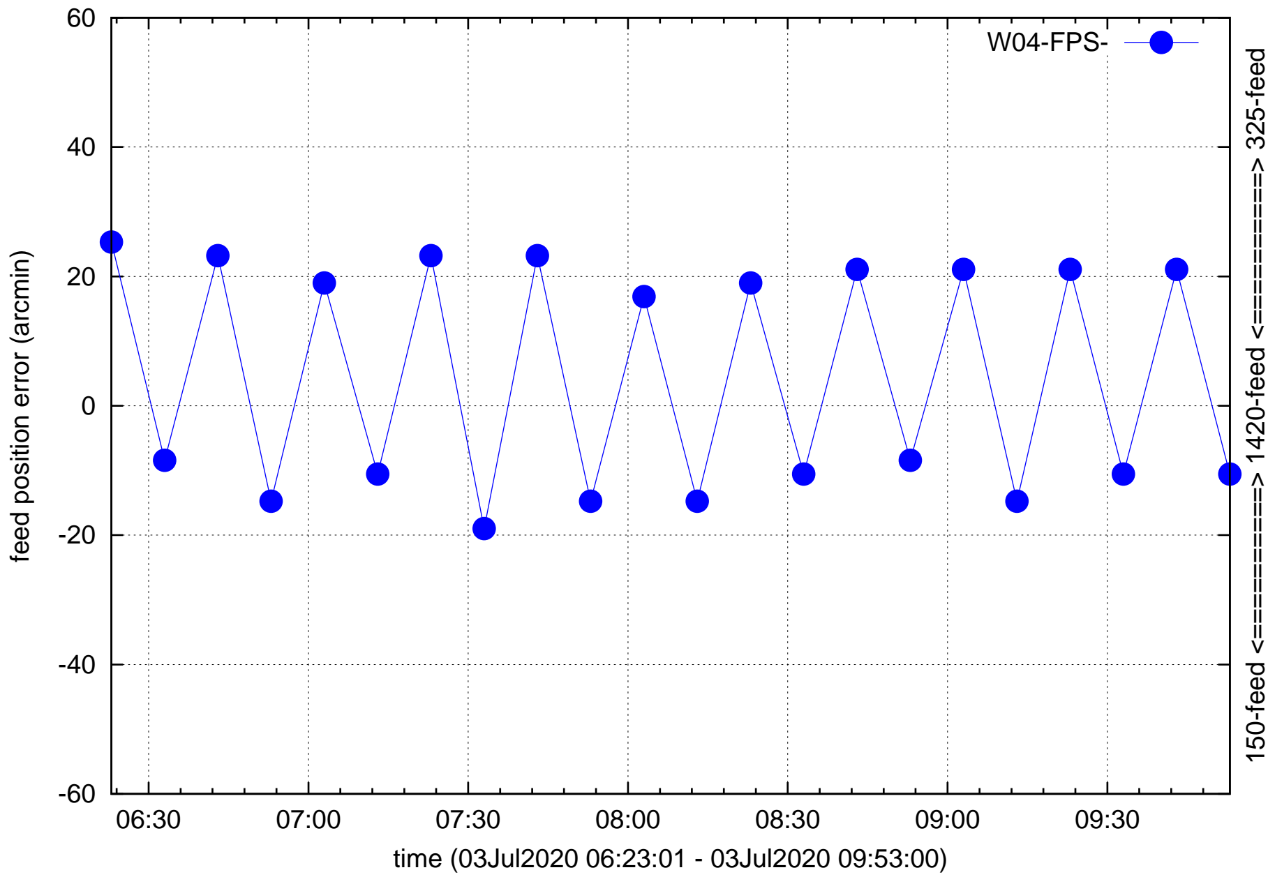
W04 feed refocusing 150=>1420, 325=>1420, ...
