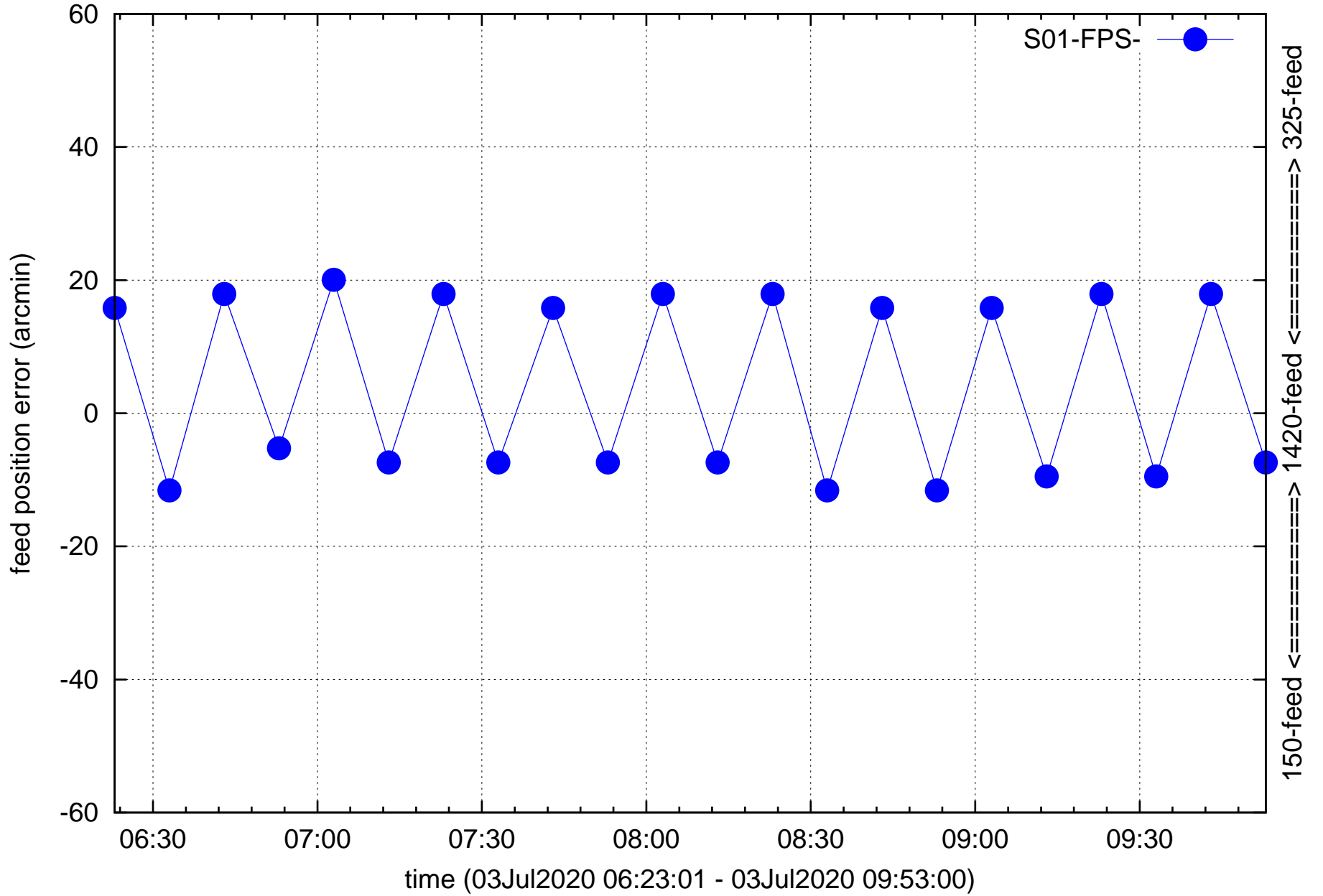
S01 feed refocusing 150=>1420, 325=>1420, ...
