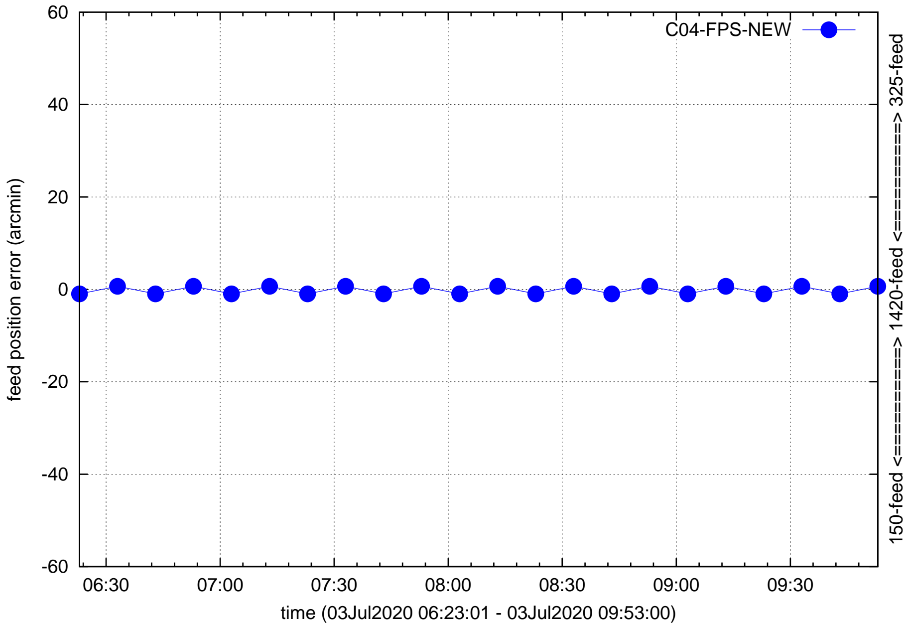
C04 feed refocusing 150=>1420, 325=>1420, ...
