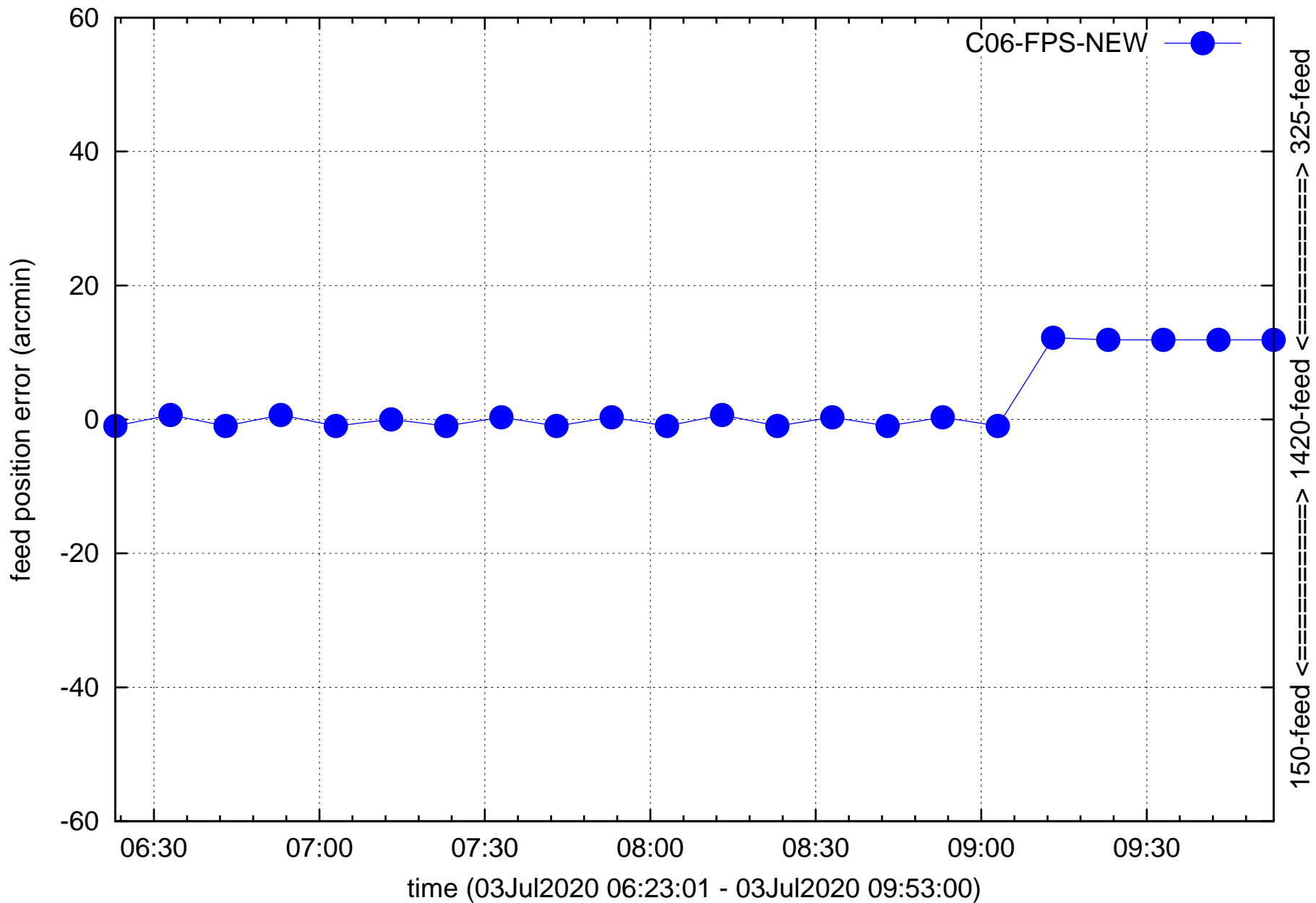
C06 feed refocusing 150=>1420, 325=>1420, ...
