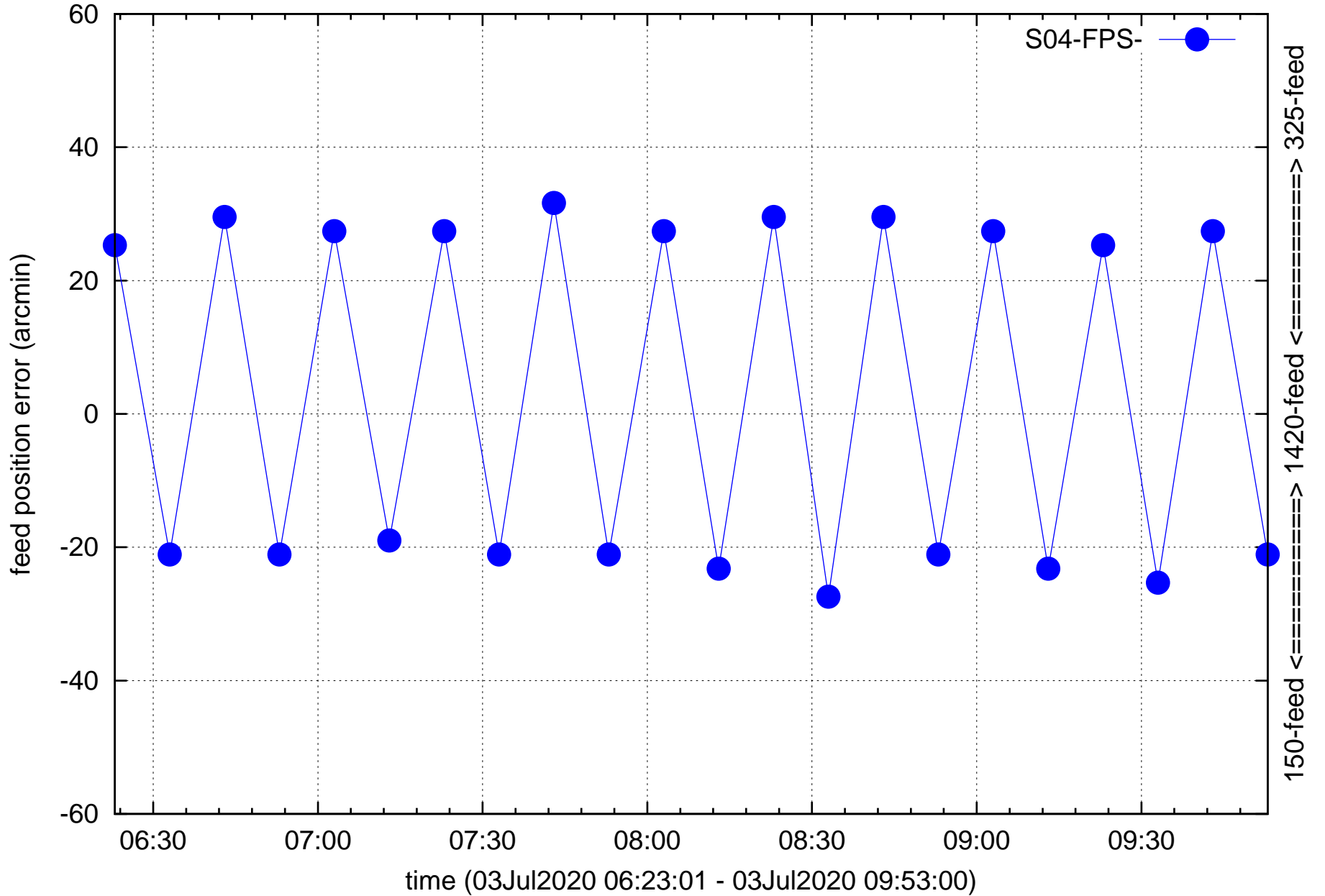
S04 feed refocusing 150=>1420, 325=>1420, ...
