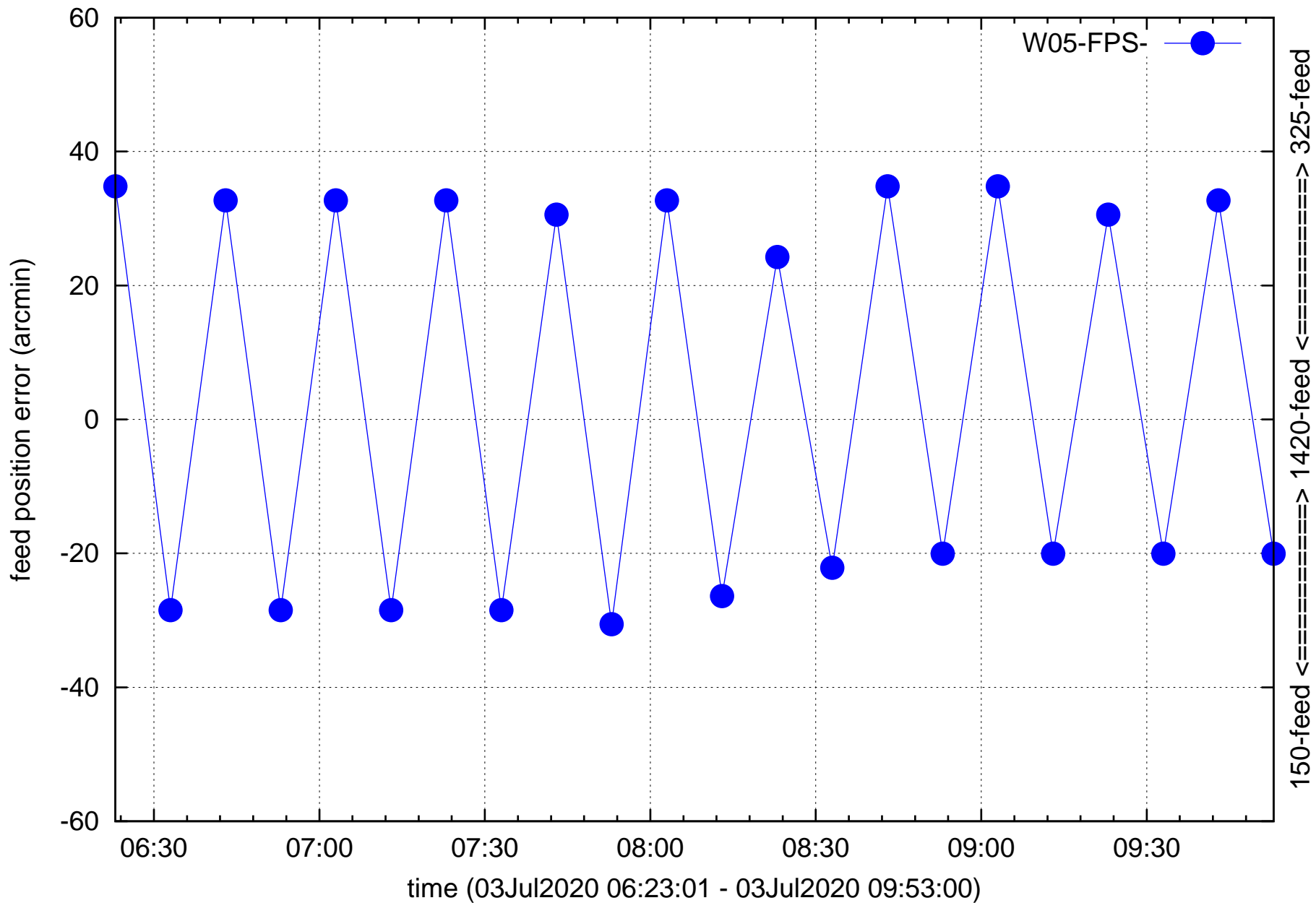
W05 feed refocusing 150=>1420, 325=>1420, ...
