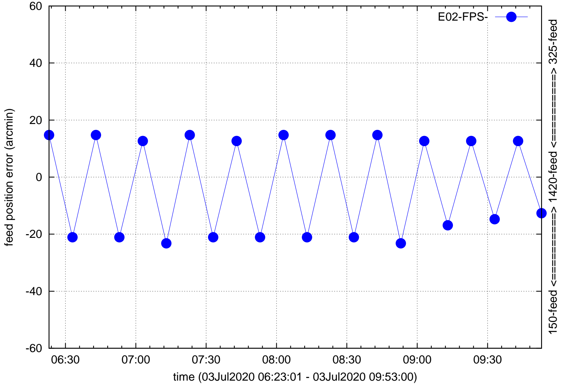
E02 feed refocusing 150=>1420, 325=>1420, ...
