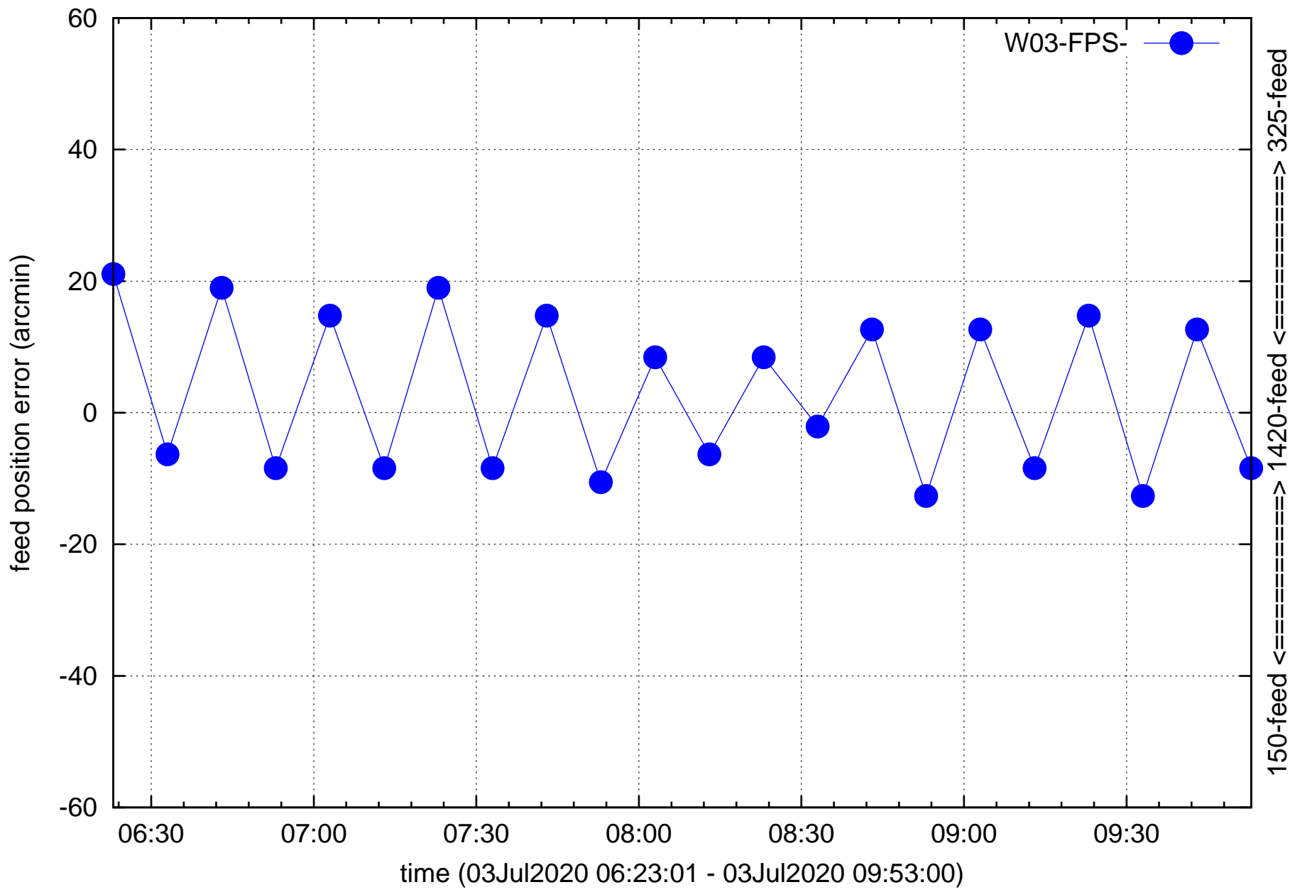
W03 feed refocusing 150=>1420, 325=>1420, ...
