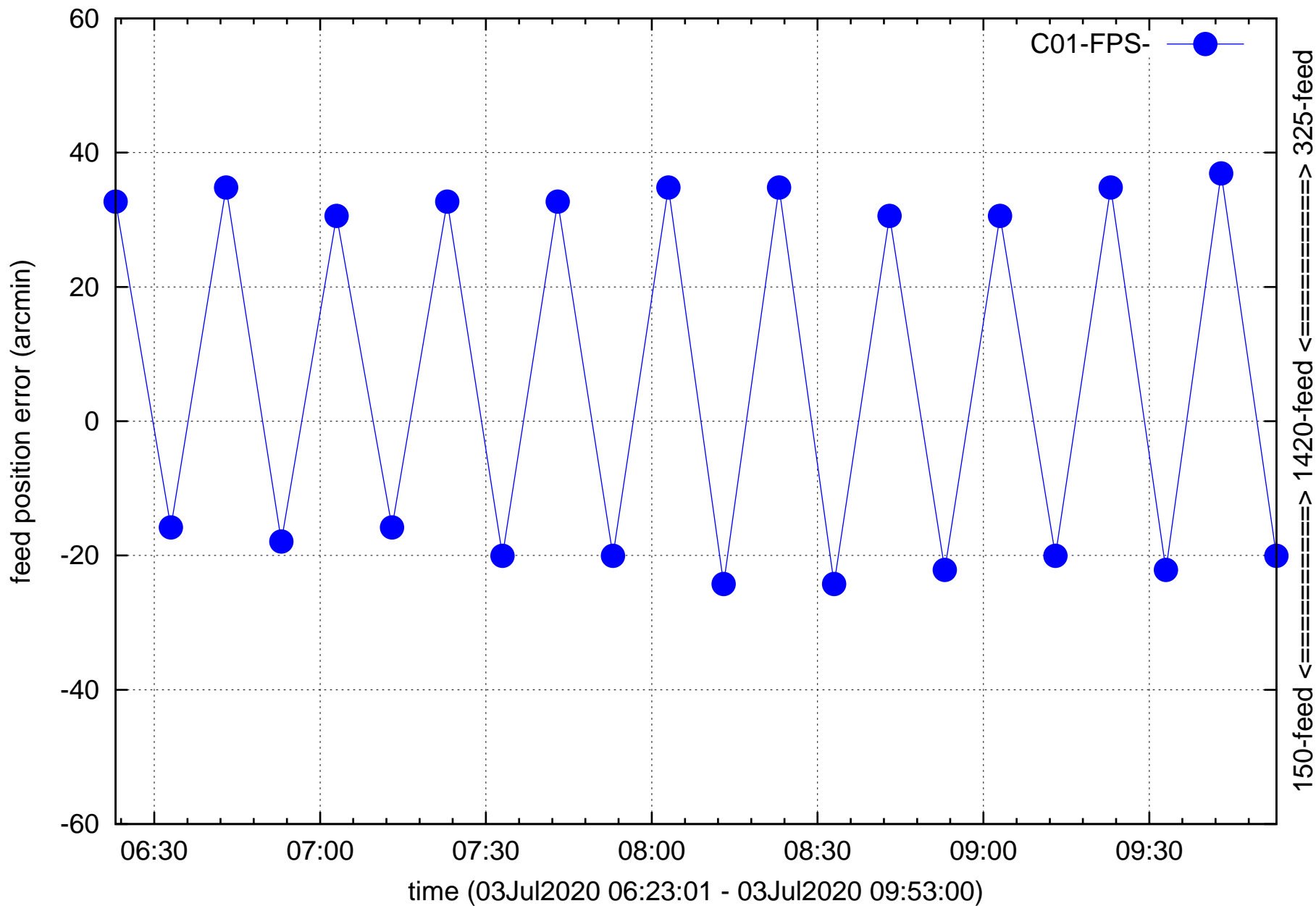
C01 feed refocusing 150=>1420, 325=>1420, ...
