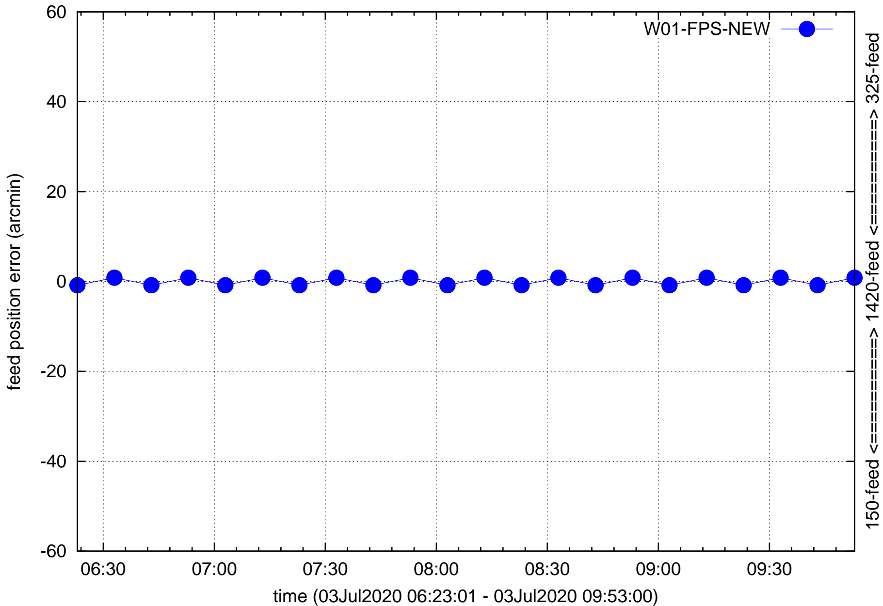
W01 feed refocusing 150=>1420, 325=>1420, ...
