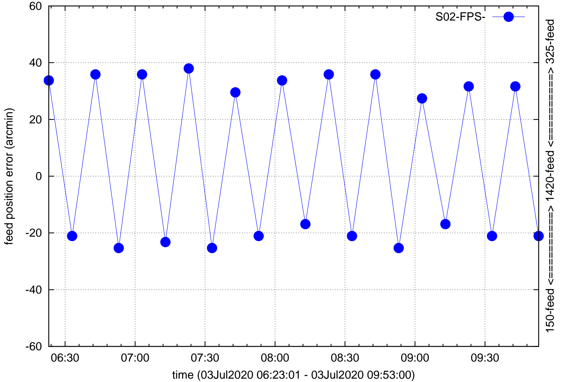
S02 feed refocusing 150=>1420, 325=>1420, ...
