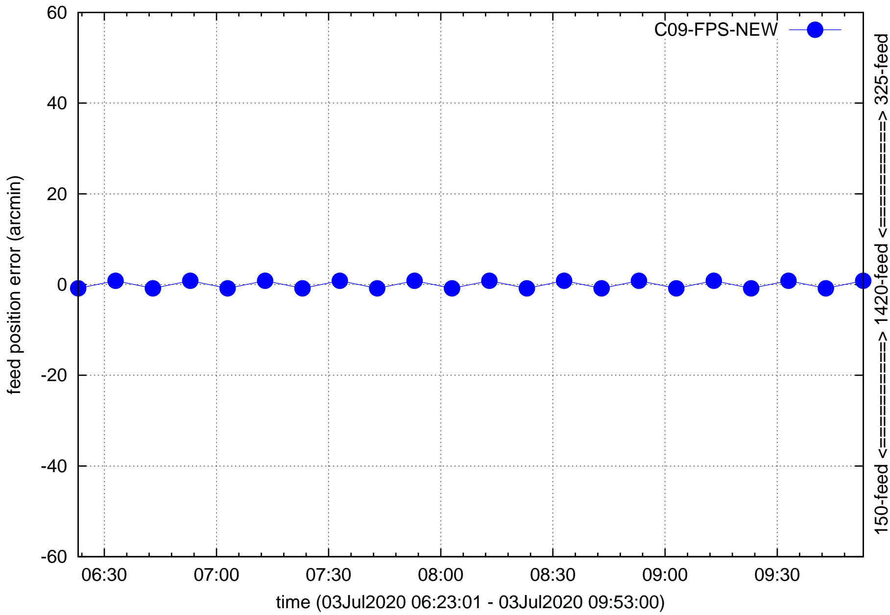
C09 feed refocusing 150=>1420, 325=>1420, ...
