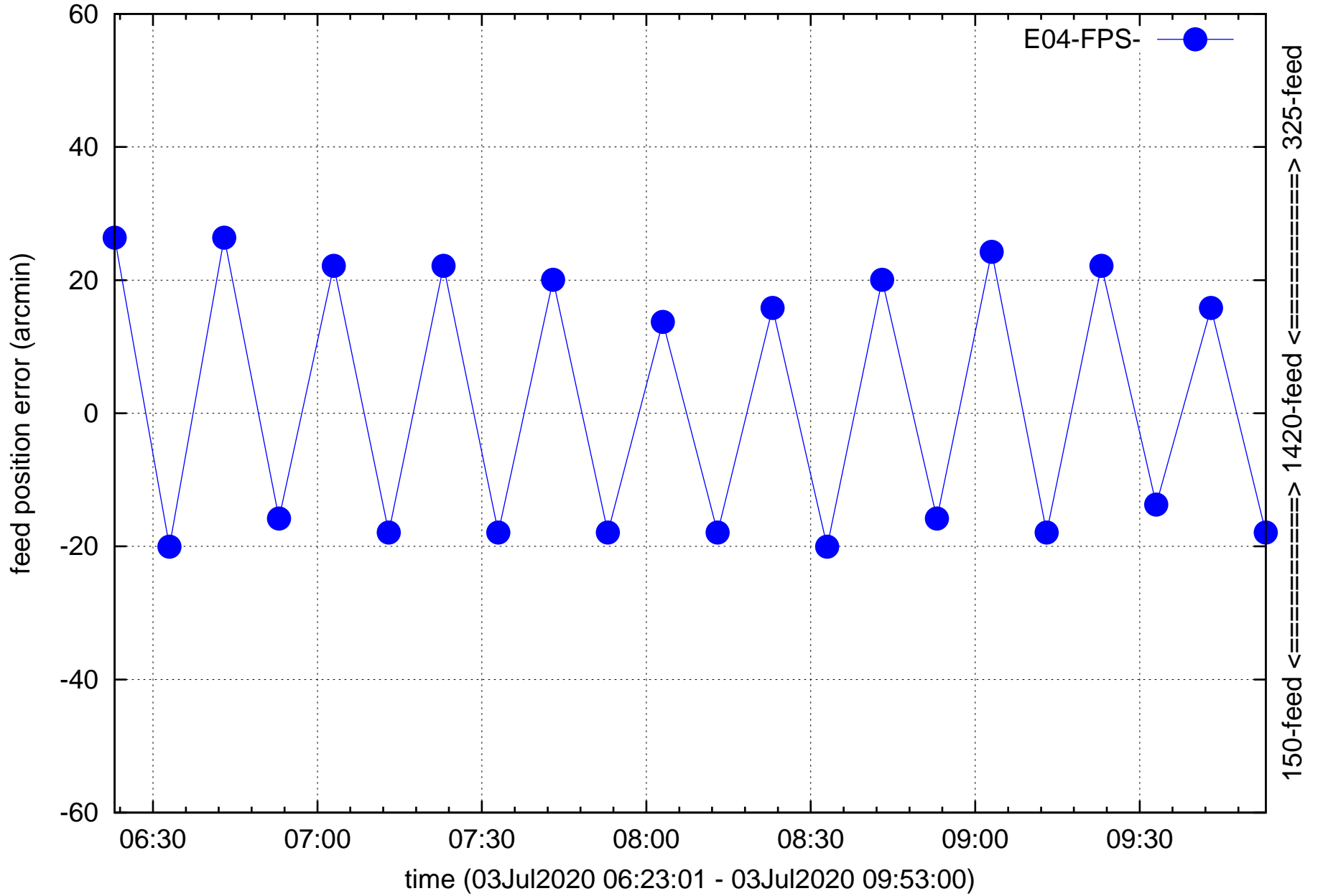
E04 feed refocusing 150=>1420, 325=>1420, ...
