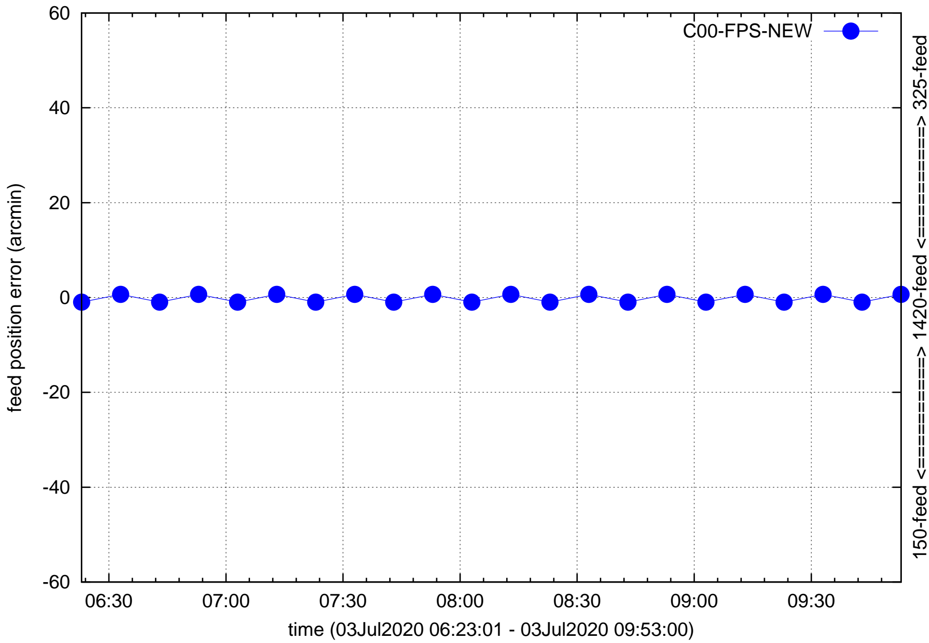
C00 feed refocusing 150=>1420, 325=>1420, ...
