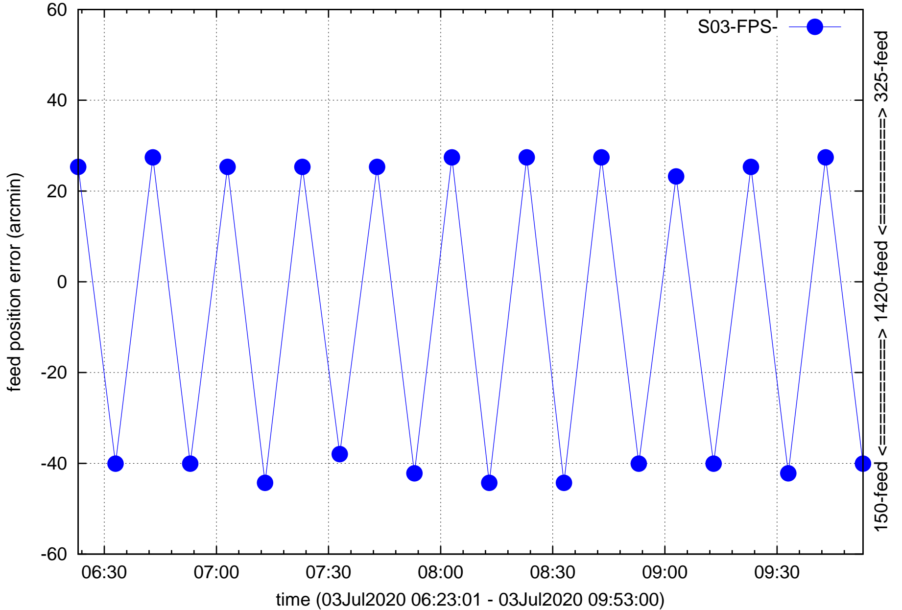
S03 feed refocusing 150=>1420, 325=>1420, ...
