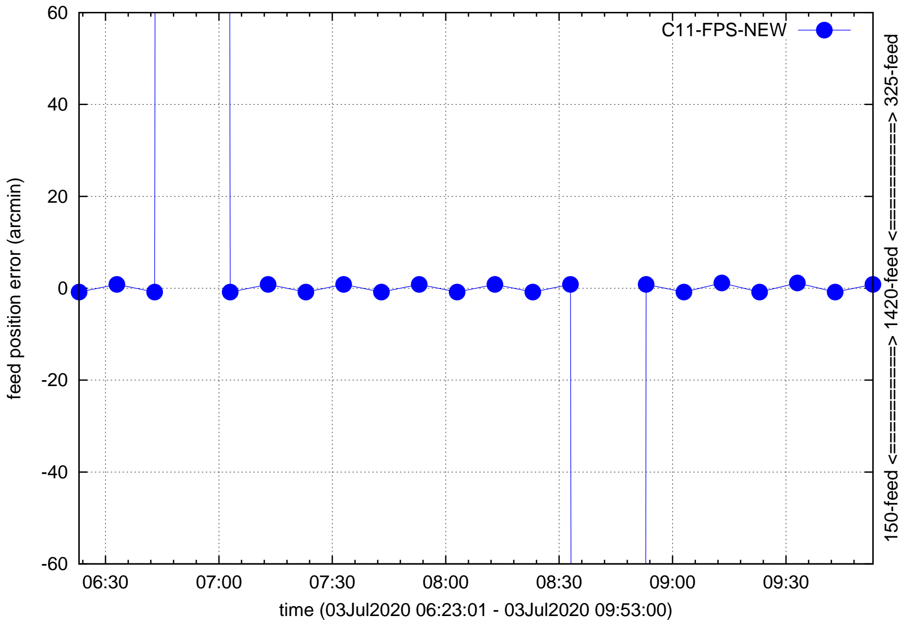
C11 feed refocusing 150=>1420, 325=>1420, ...
