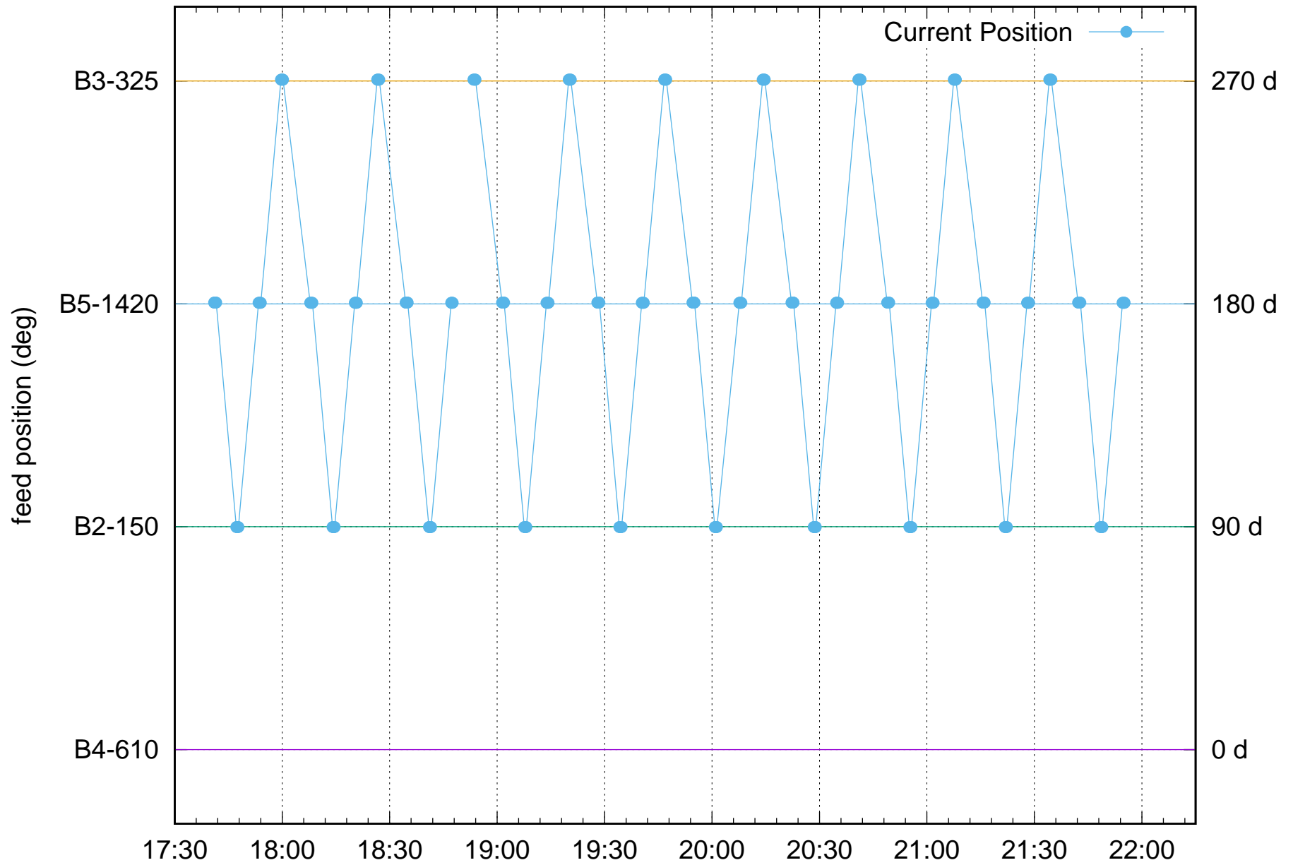
FPS Rotation position: C01-NEW-FPS 08Feb2022
