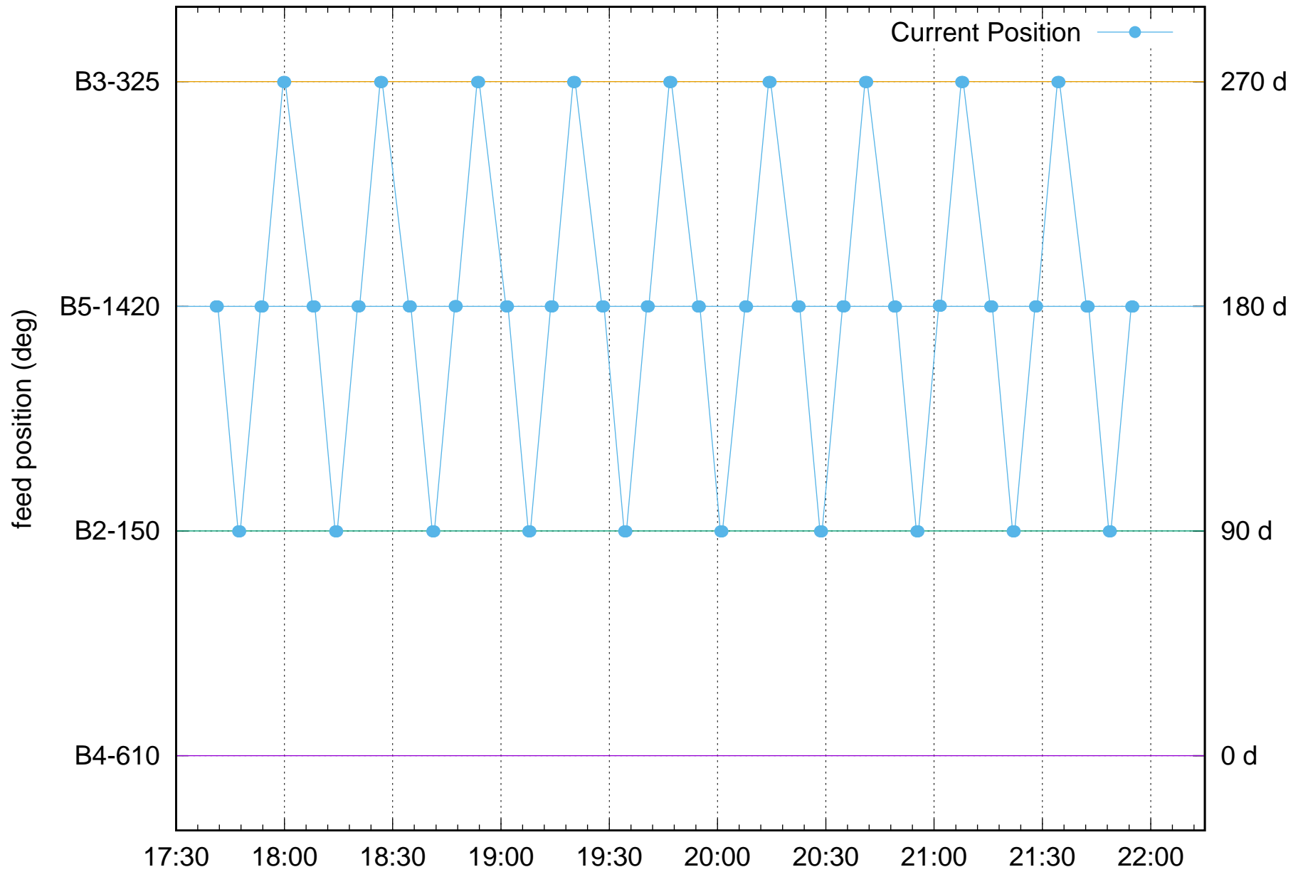
FPS Rotation position: W03-NEW-FPS 08Feb2022
