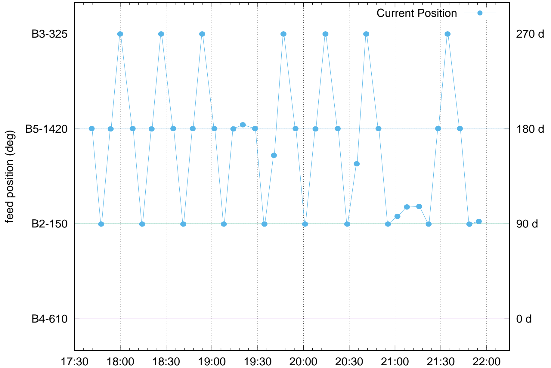
FPS Rotation position: S01-NEW-FPS 08Feb2022
