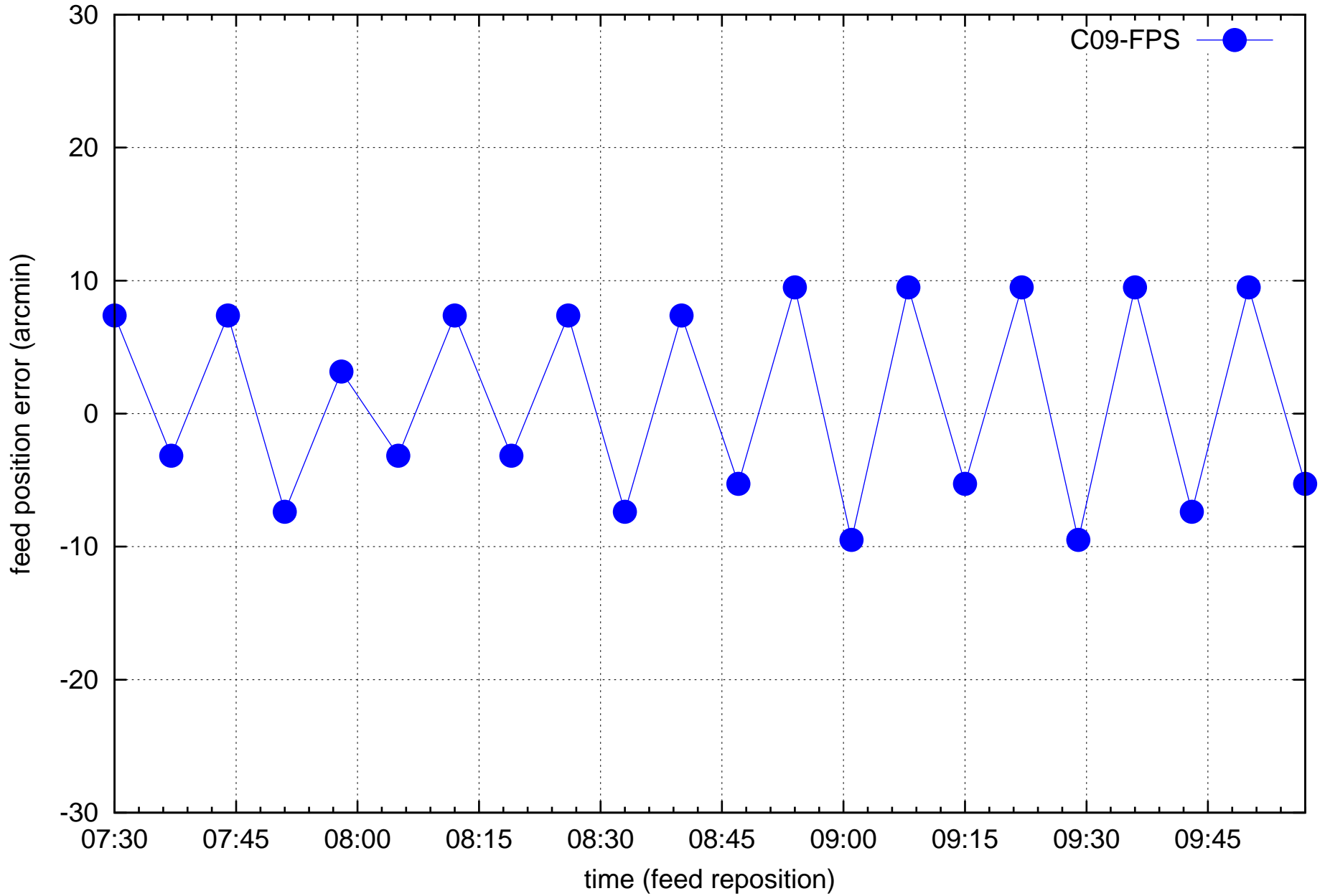
C09 feed refocusing
