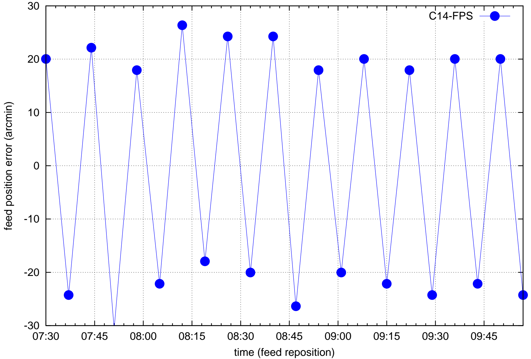
C14 feed refocusing
