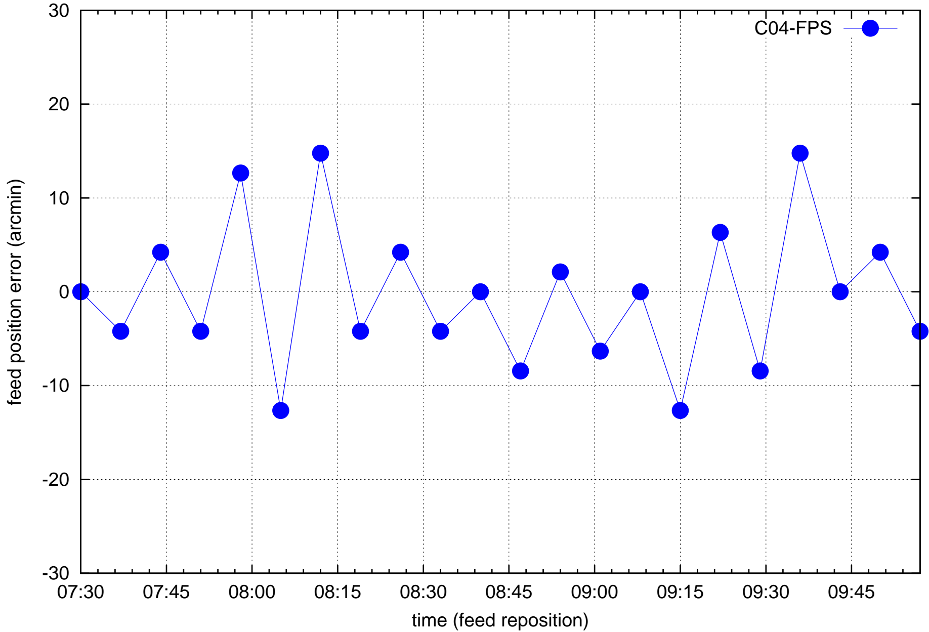
C04 feed refocusing
