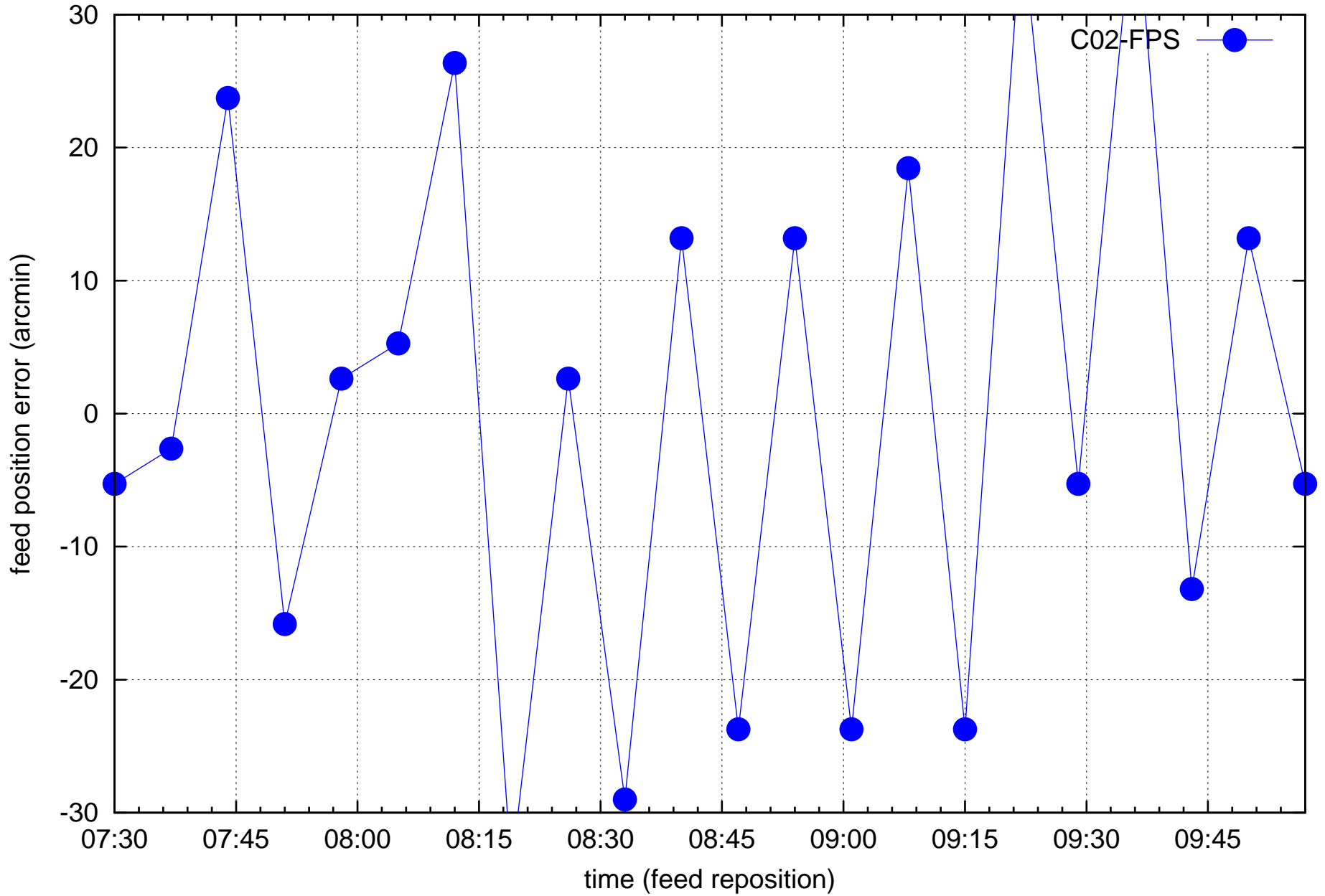
C02 feed refocusing
