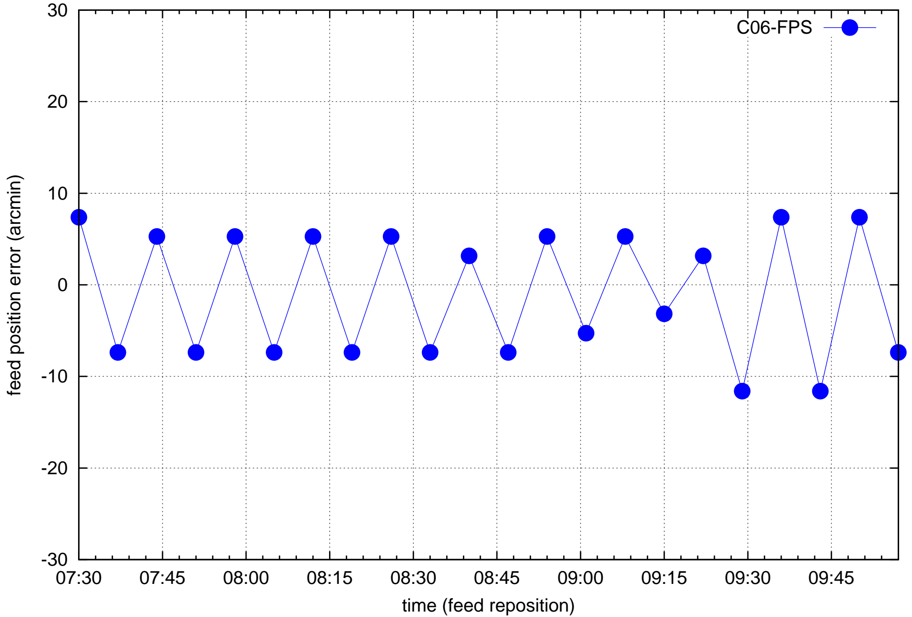
C06 feed refocusing
