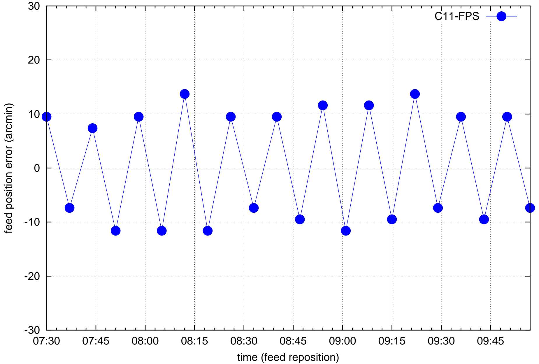
C11 feed refocusing
