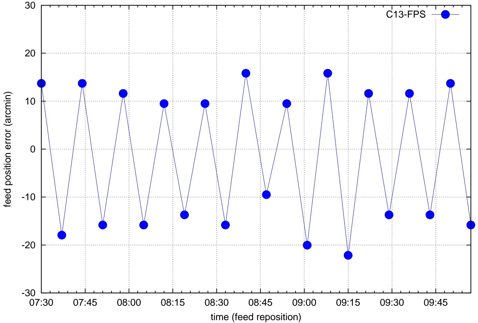
C13 feed refocusing
