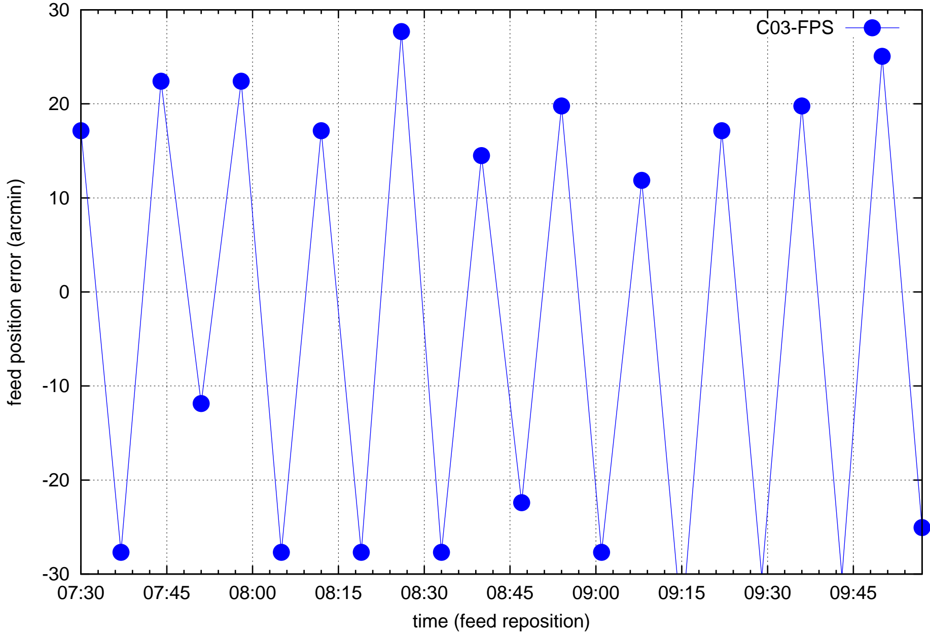
C03 feed refocusing
