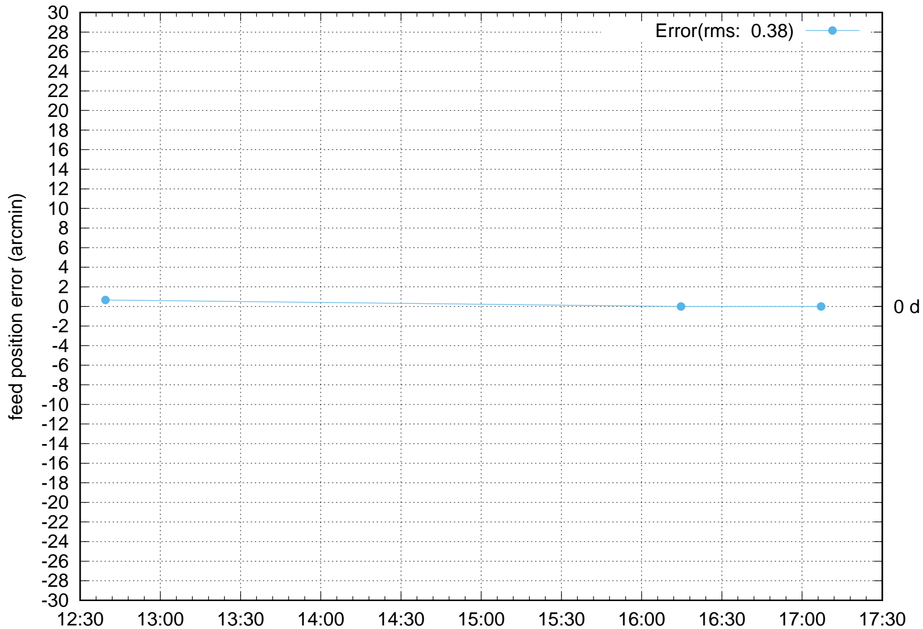
FPS Rotation error: E02-NEW-FPS fps 2 1mar2022.log
