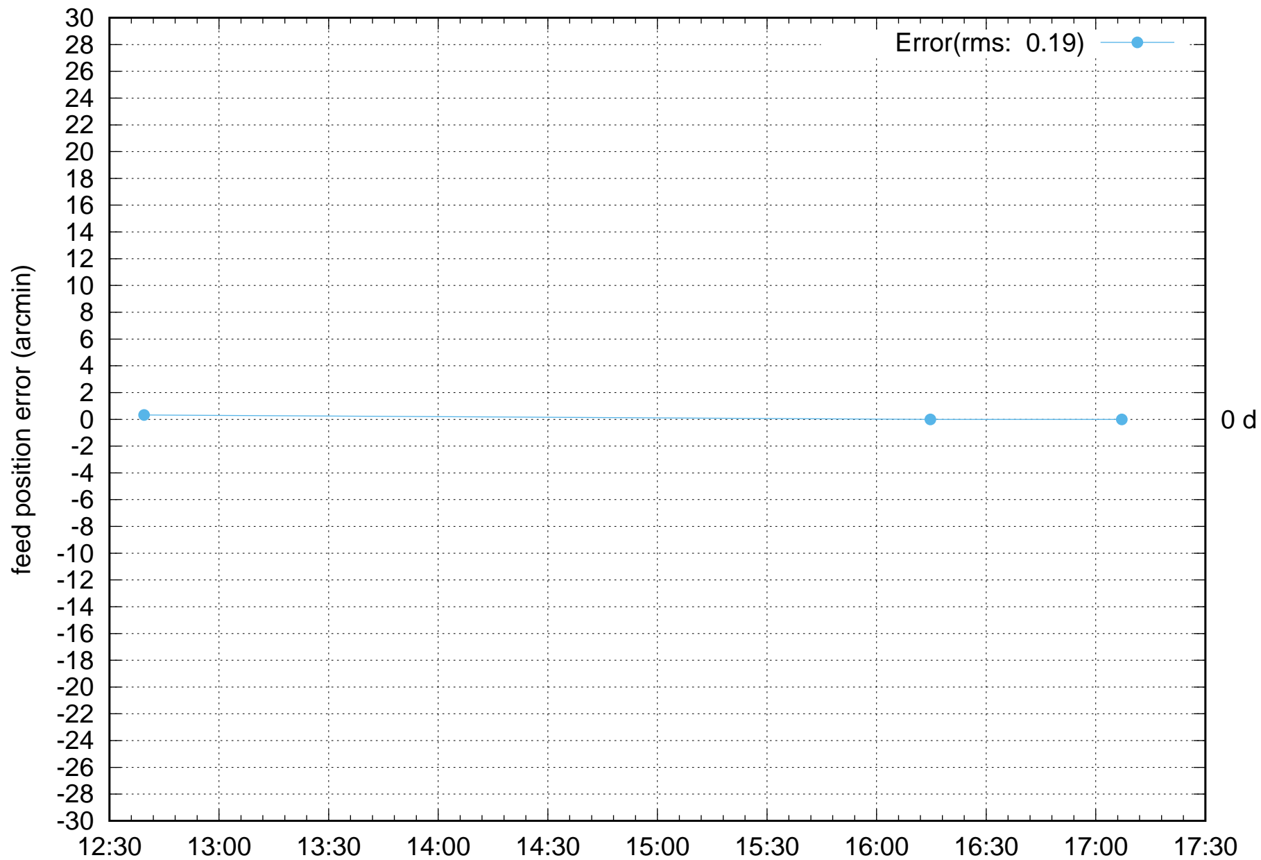
FPS Rotation error: E05-NEW-FPS fps 2 1mar2022.log
