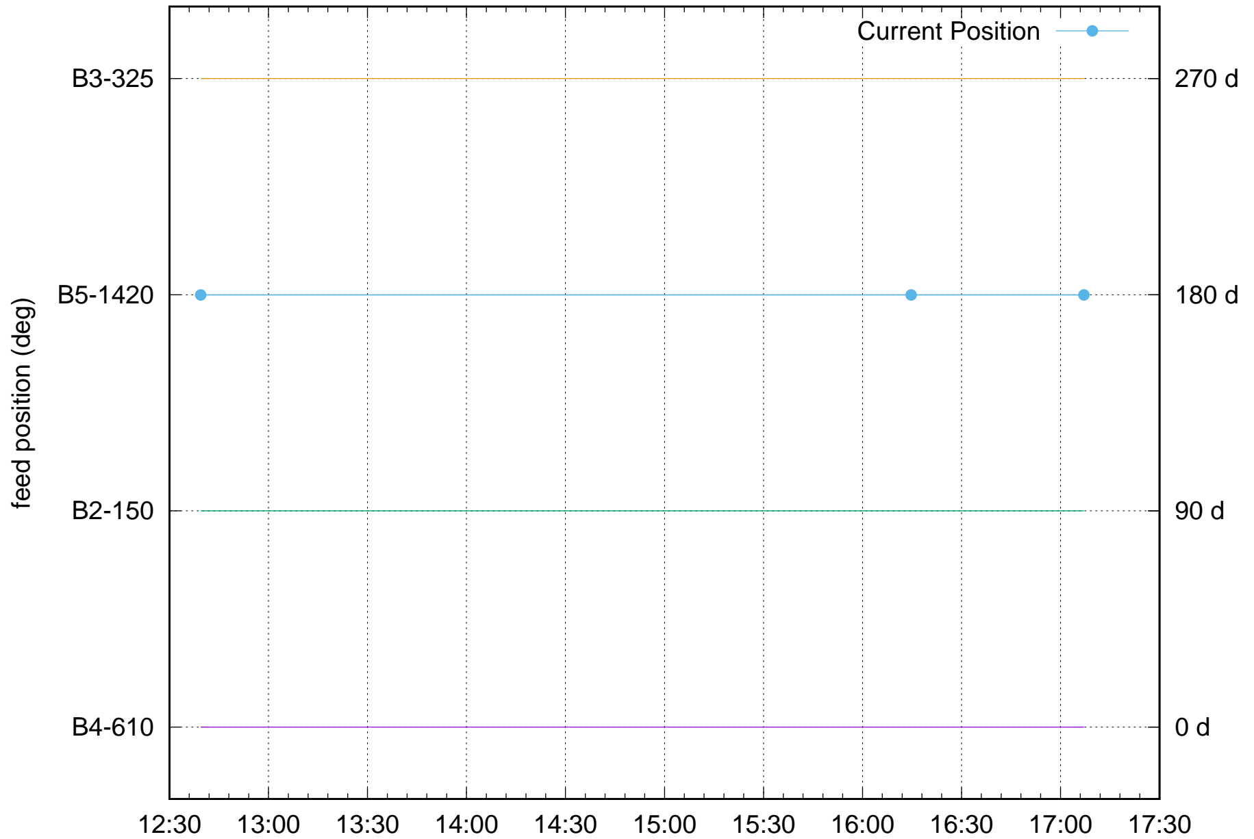
FPS Rotation position: W01-NEW-FPS fps 2 1mar2022.log
