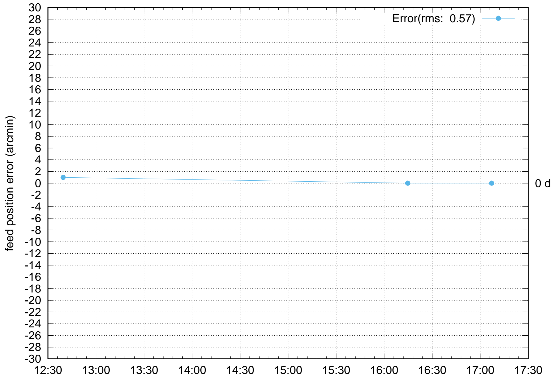
FPS Rotation error: W01-NEW-FPS fps 2 1 mar2022.log
