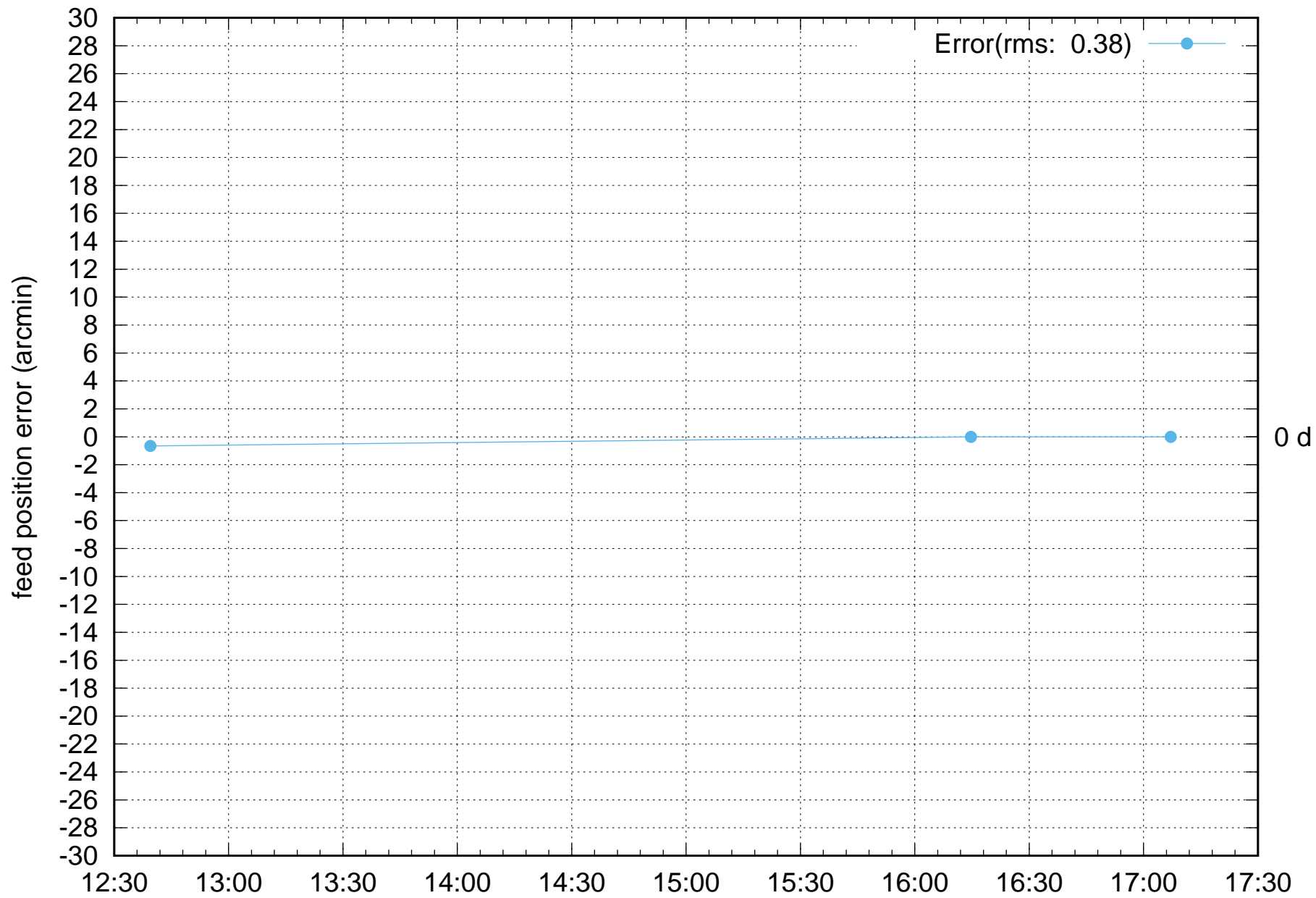
FPS Rotation error: C09-NEW-FPS fps 2 1mar2022.log
