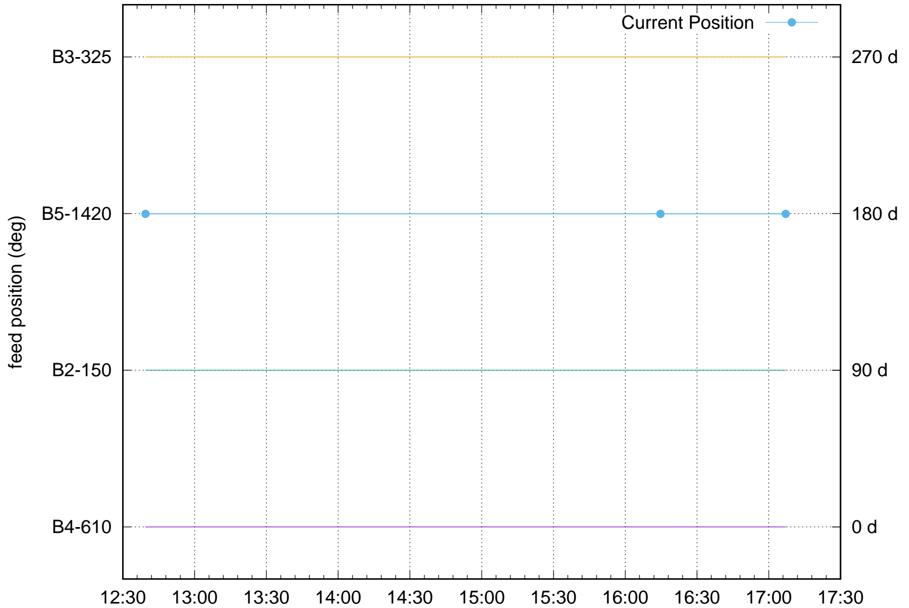
FPS Rotation position: C10-NEW-FPS fps 2 1mar2022.log
