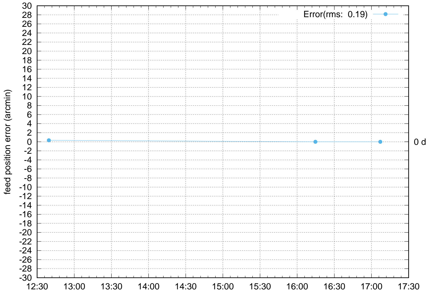
FPS Rotation error: W02-NEW-FPS fps 2 1 mar2022.log
