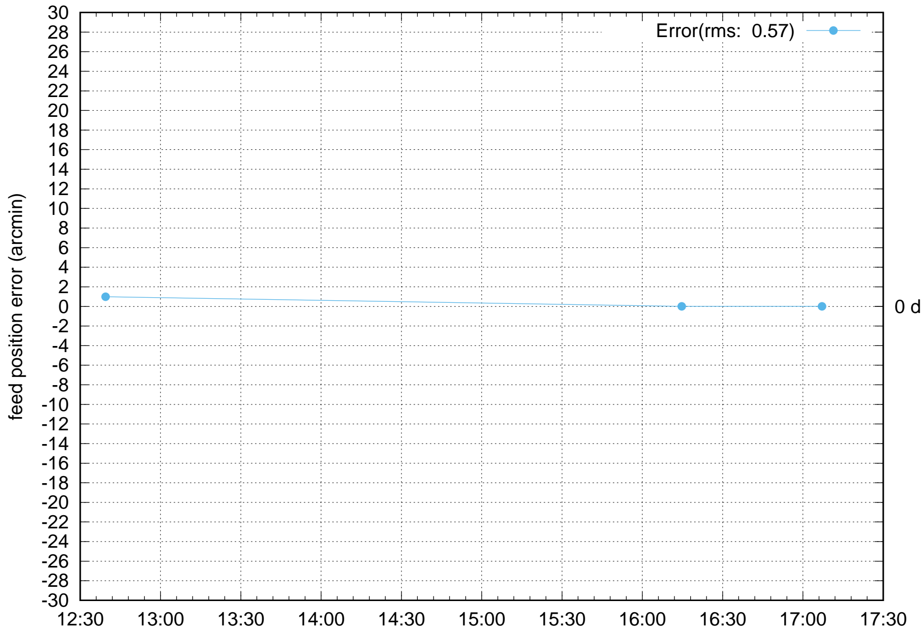
FPS Rotation error: C11-NEW-FPS fps 2 1mar2022.log
