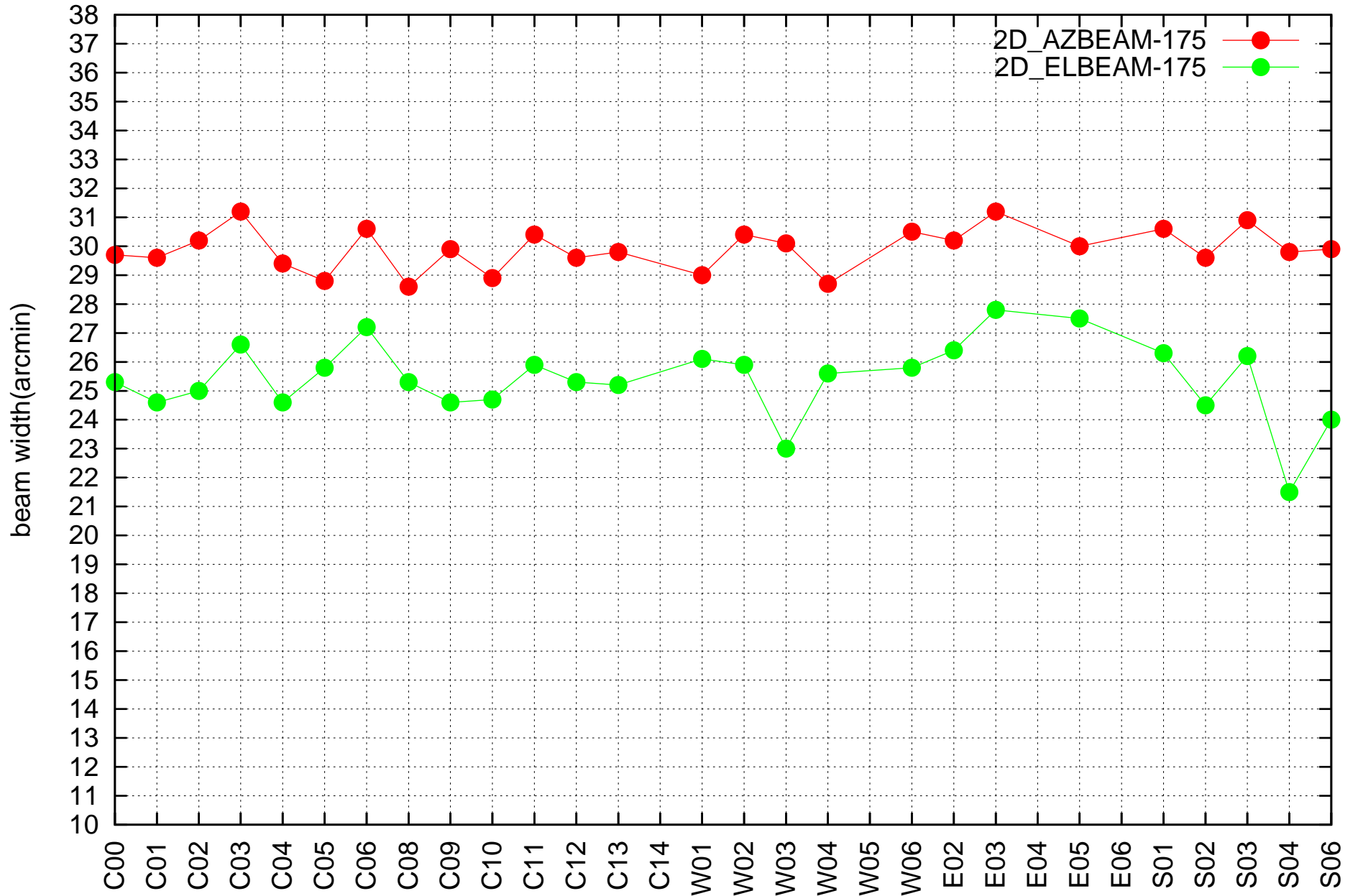
1170 MHz. 17 points
