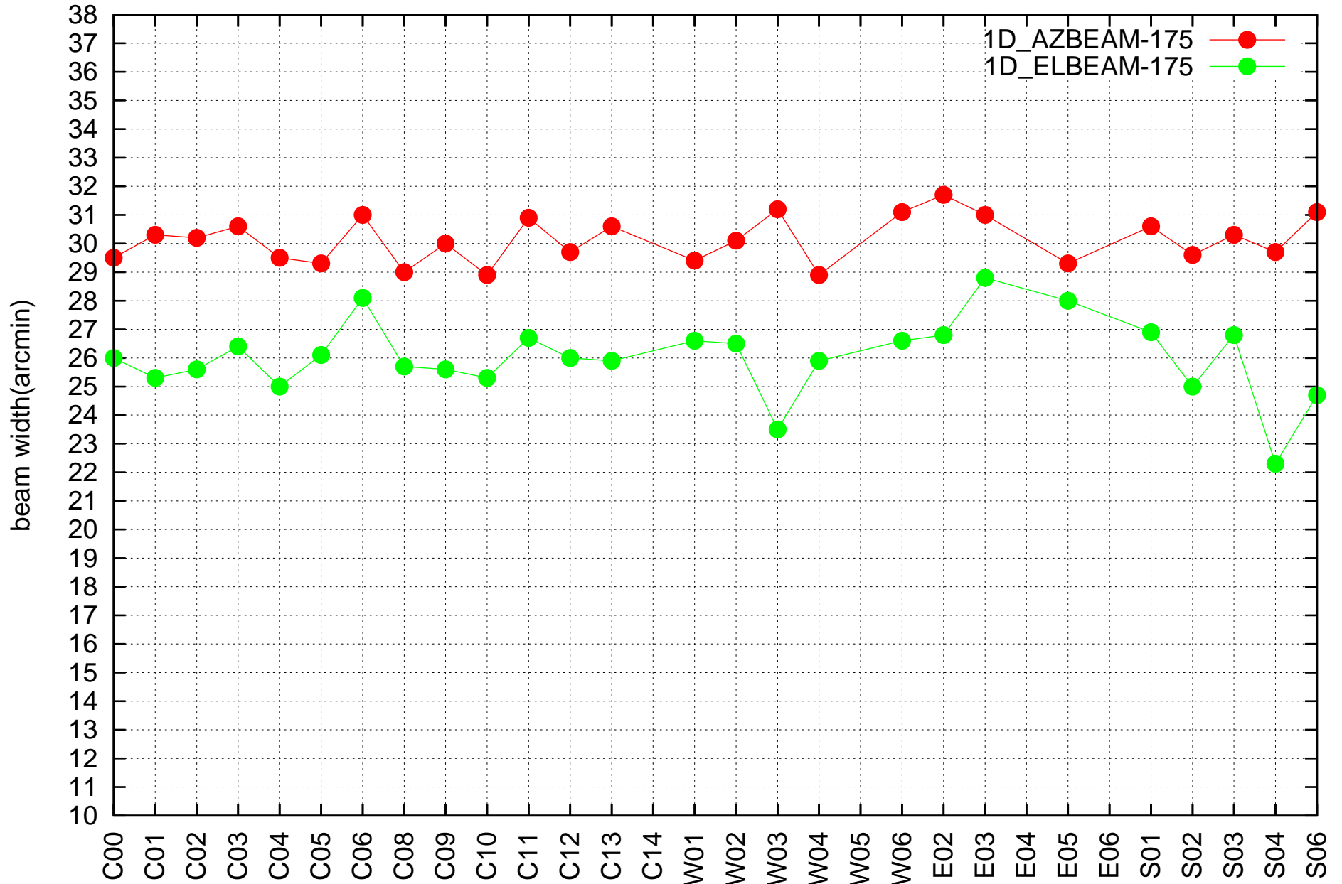
1170 MHz. 17 points
