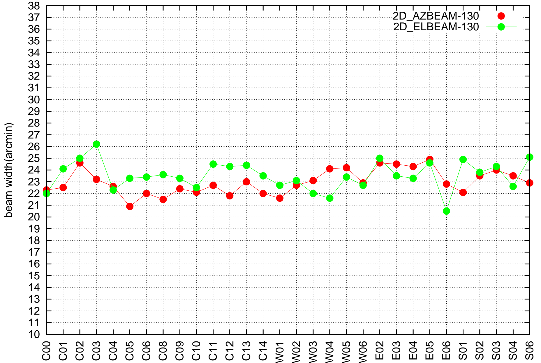
1390 MHz. 9 points
