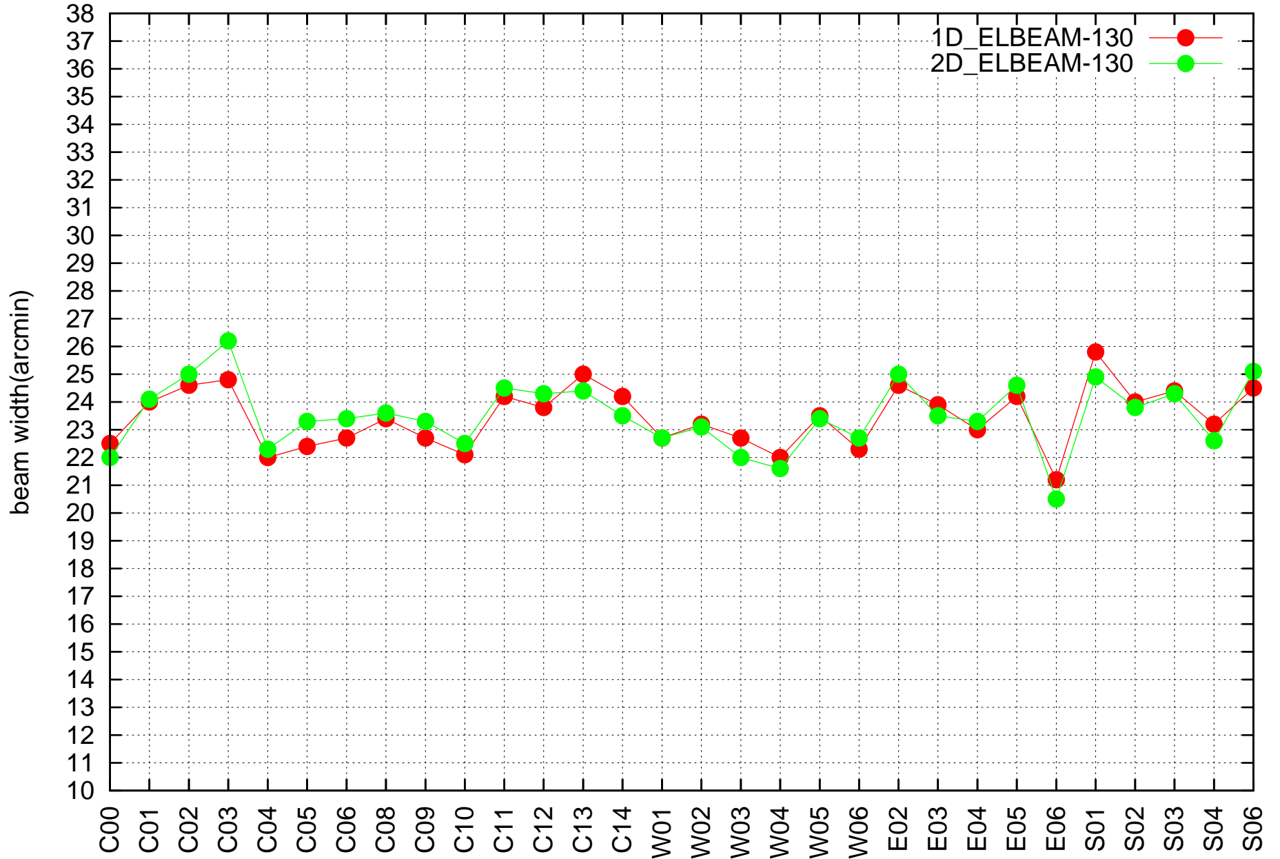
1390 MHz. 9 points
