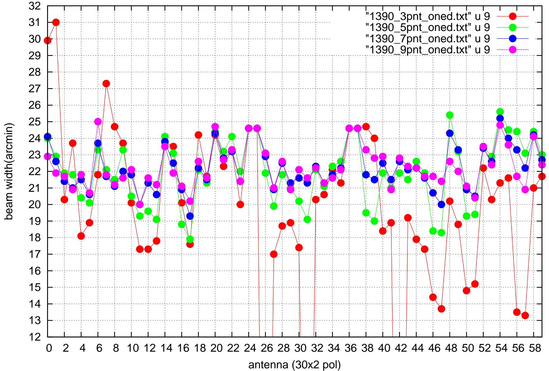
EL beam widths at 3, 5, 7 and 9 grid point 1D fit
