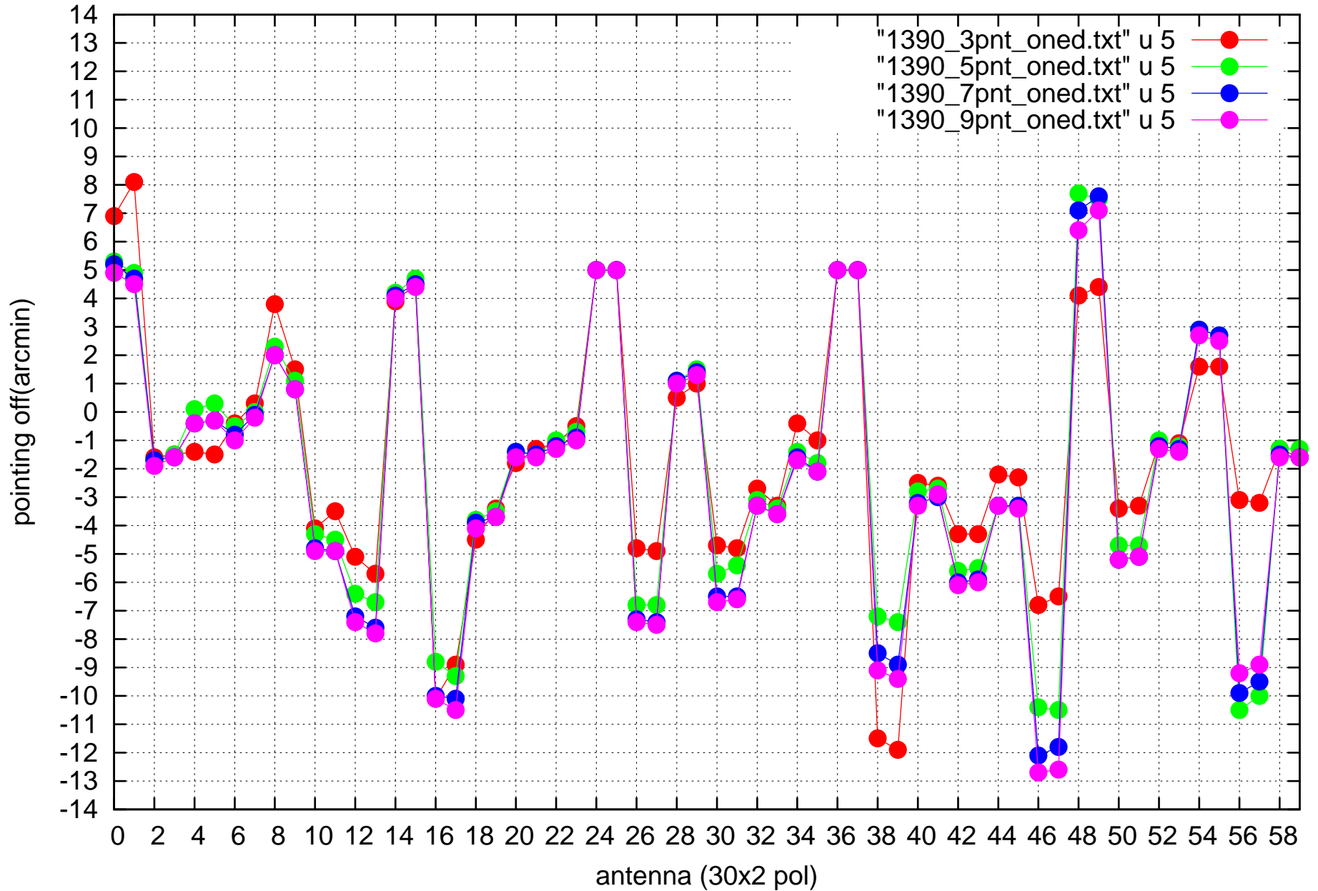
EL pointing offsets at 3, 5, 7 and 9 grid point 1D fit
