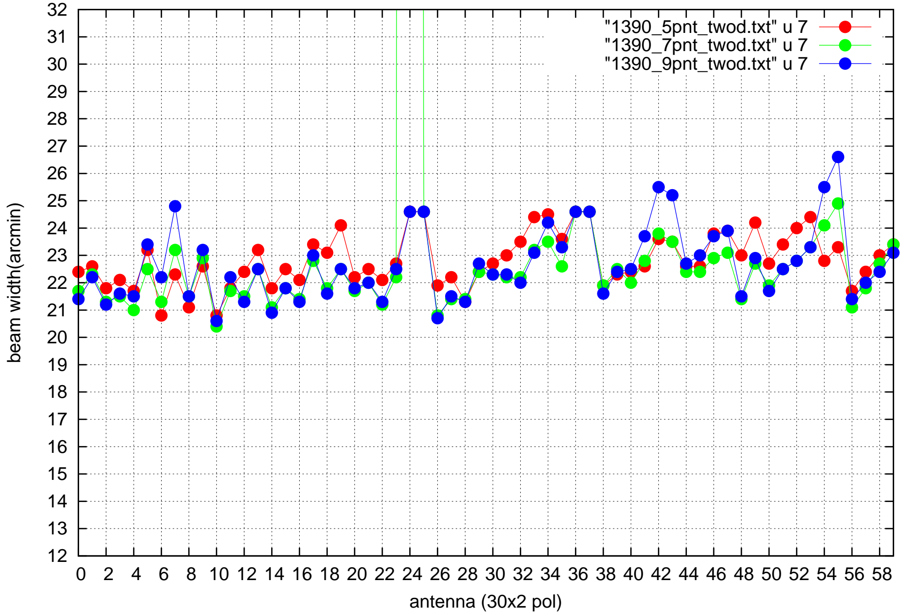
AZ beam widths at 5, 7 and 9 grid point 2D fit
