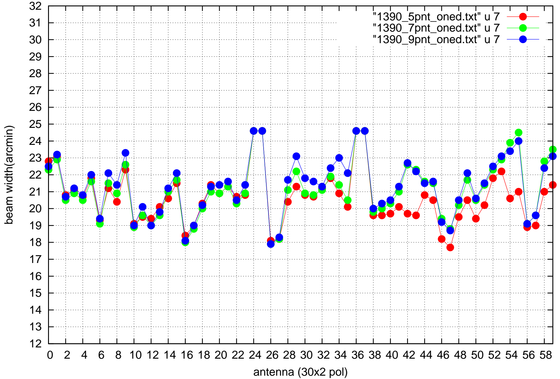
AZ beam widths at 5, 7 and 9 grid point 1D fit
