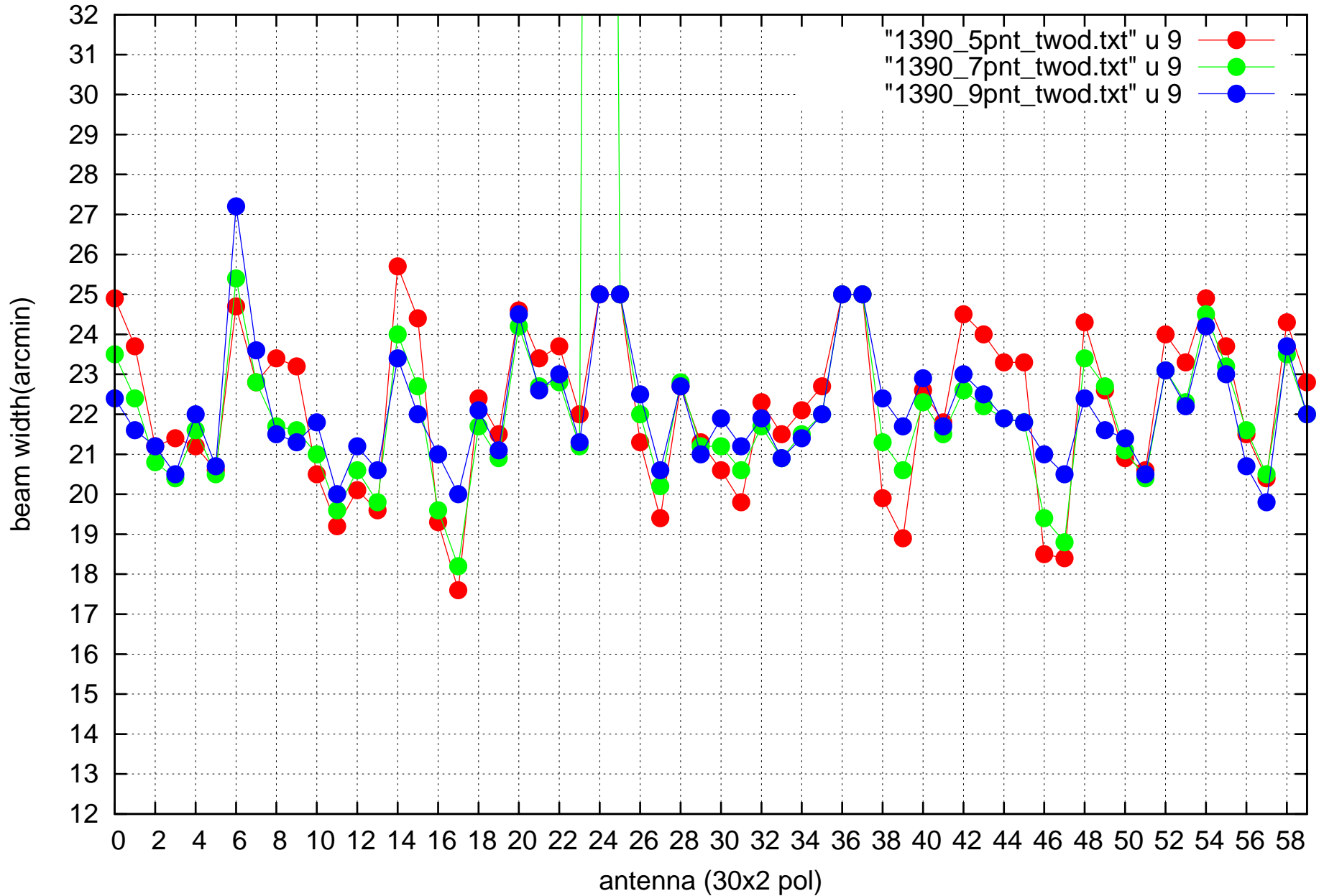
EL beam widths at 5, 7 and 9 grid point 2D fit
