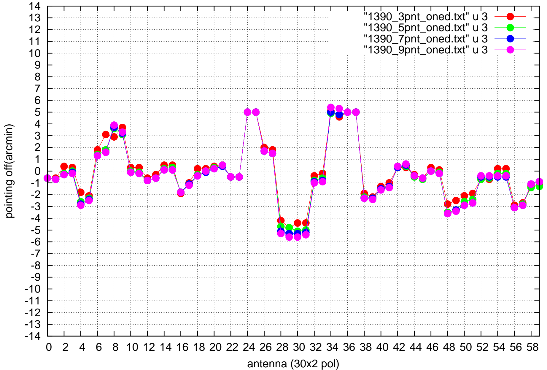
AZ pointing offsets at 3, 5, 7 and 9 grid point 1D fit
