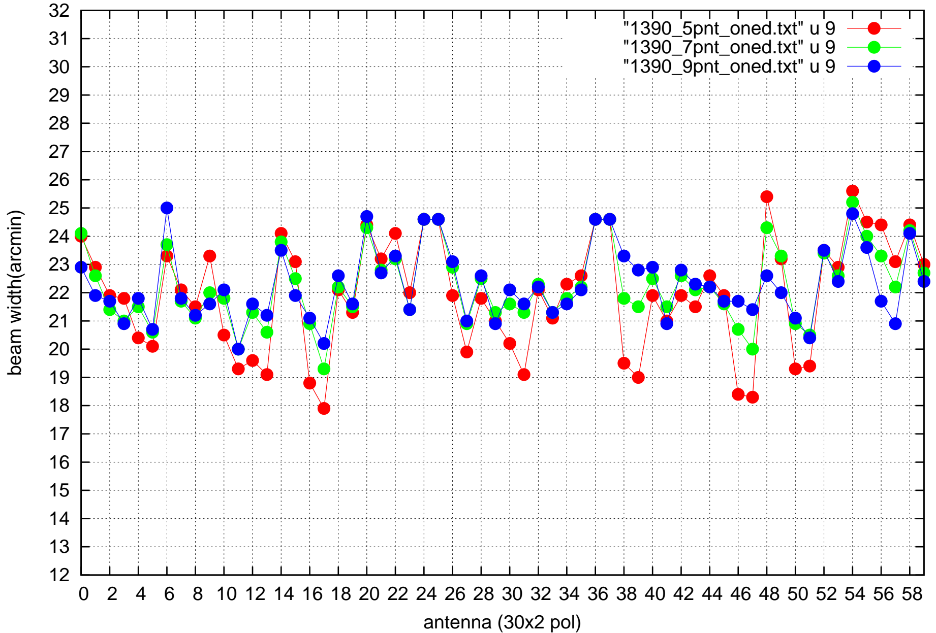
EL beam widths at 5, 7 and 9 grid point 1D fit
