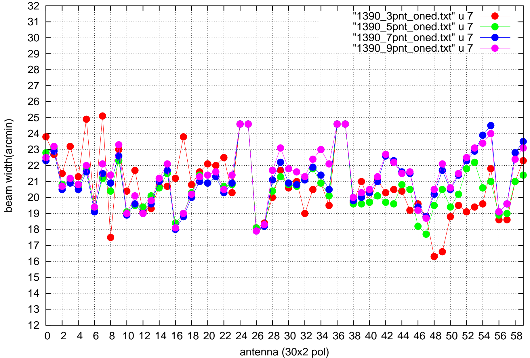
AZ beam widths at 3, 5, 7 and 9 grid point 1D fit
