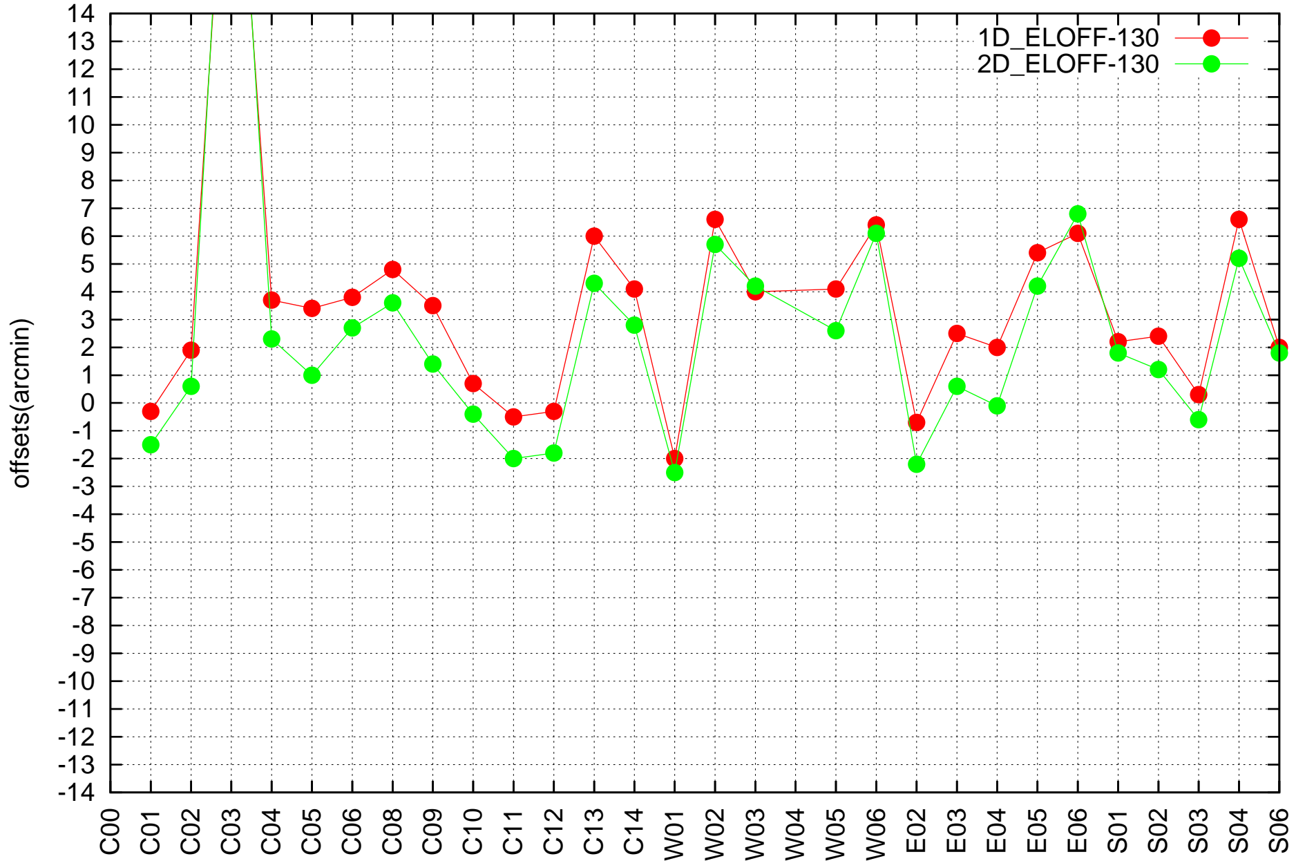
325 MHz. 13 points
