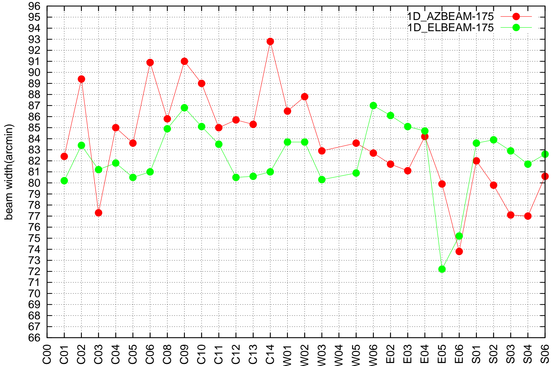
325 MHz. 13 points
