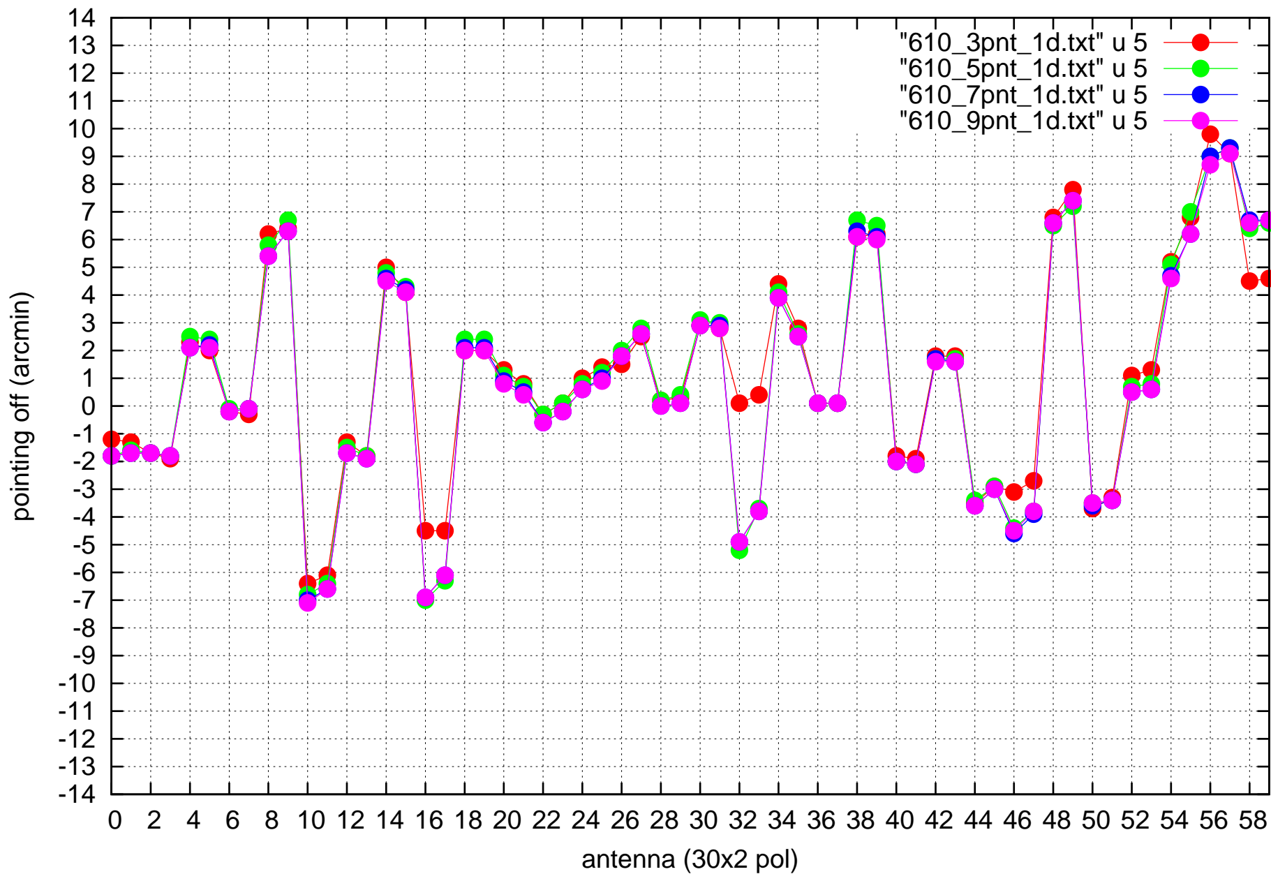
EL pointing offsets at 3, 5, 7 and 9 grid point 1D fit
