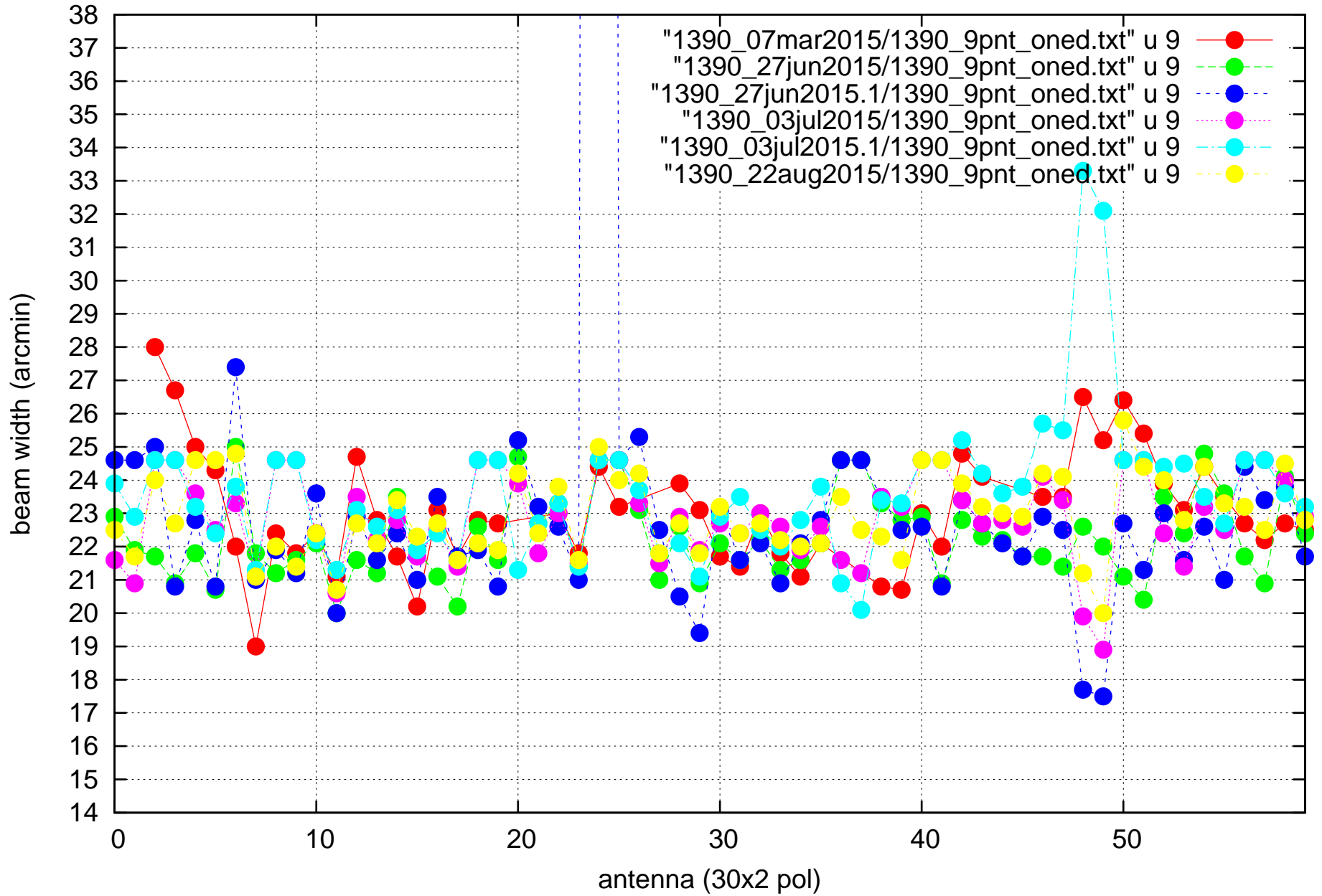
AZ beam width @ 1D
