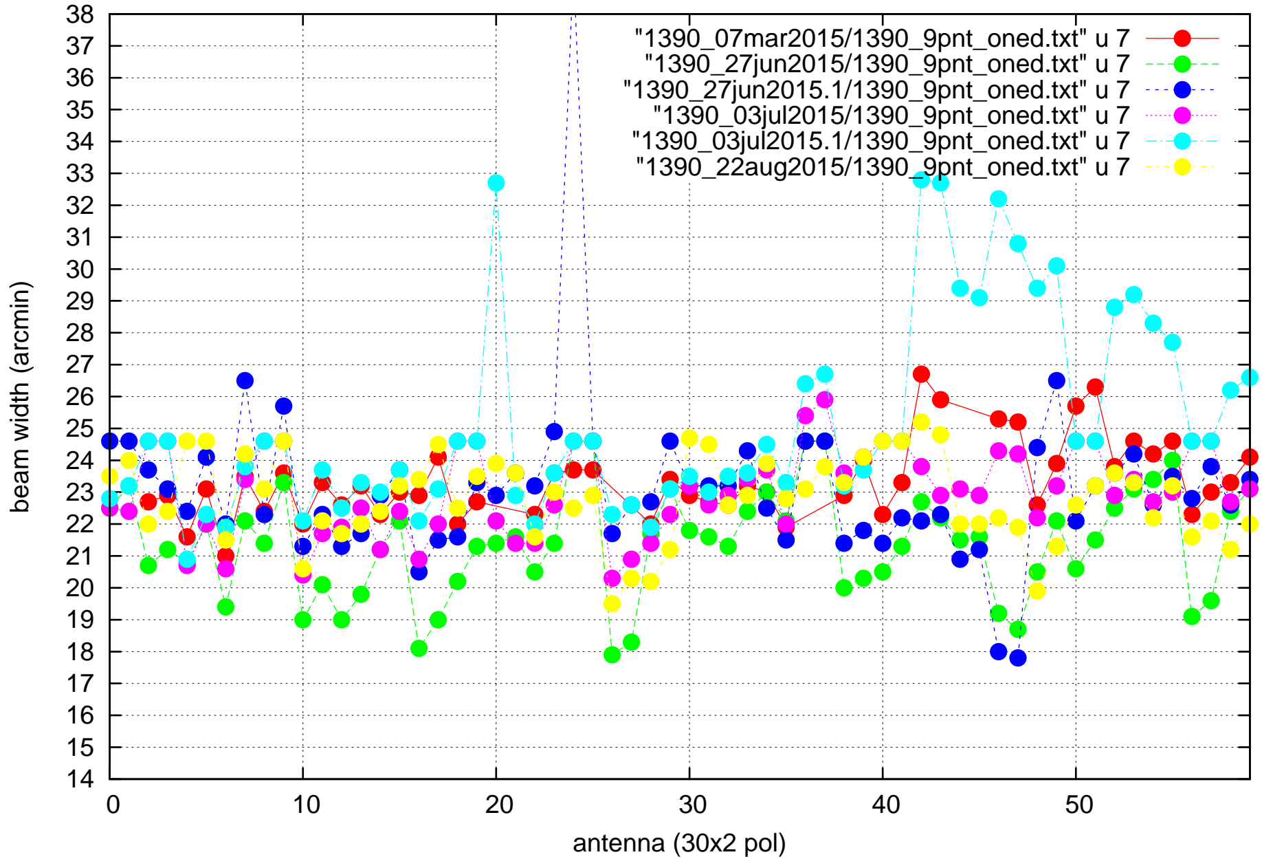
EL beam width @ 1D
