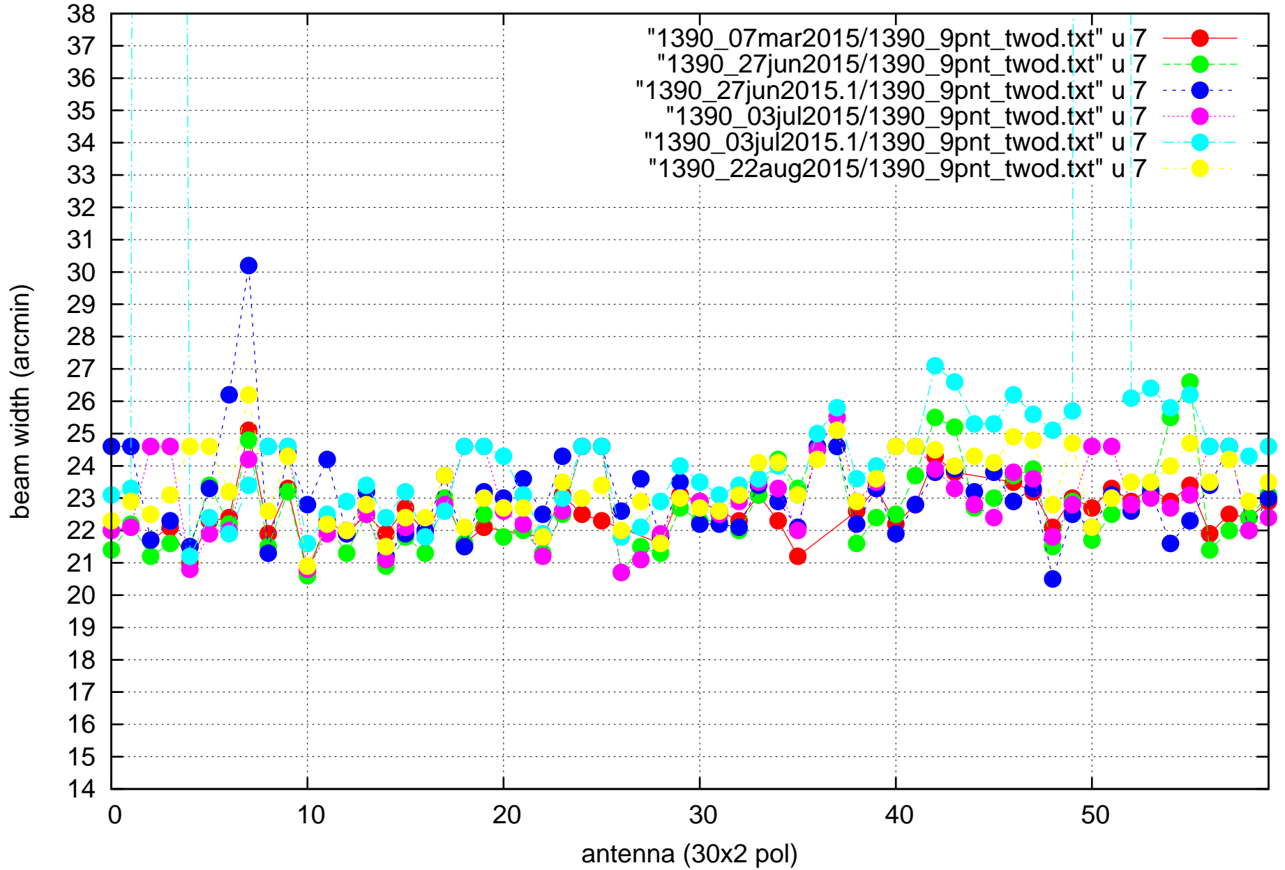
EL beam width @ 2D
